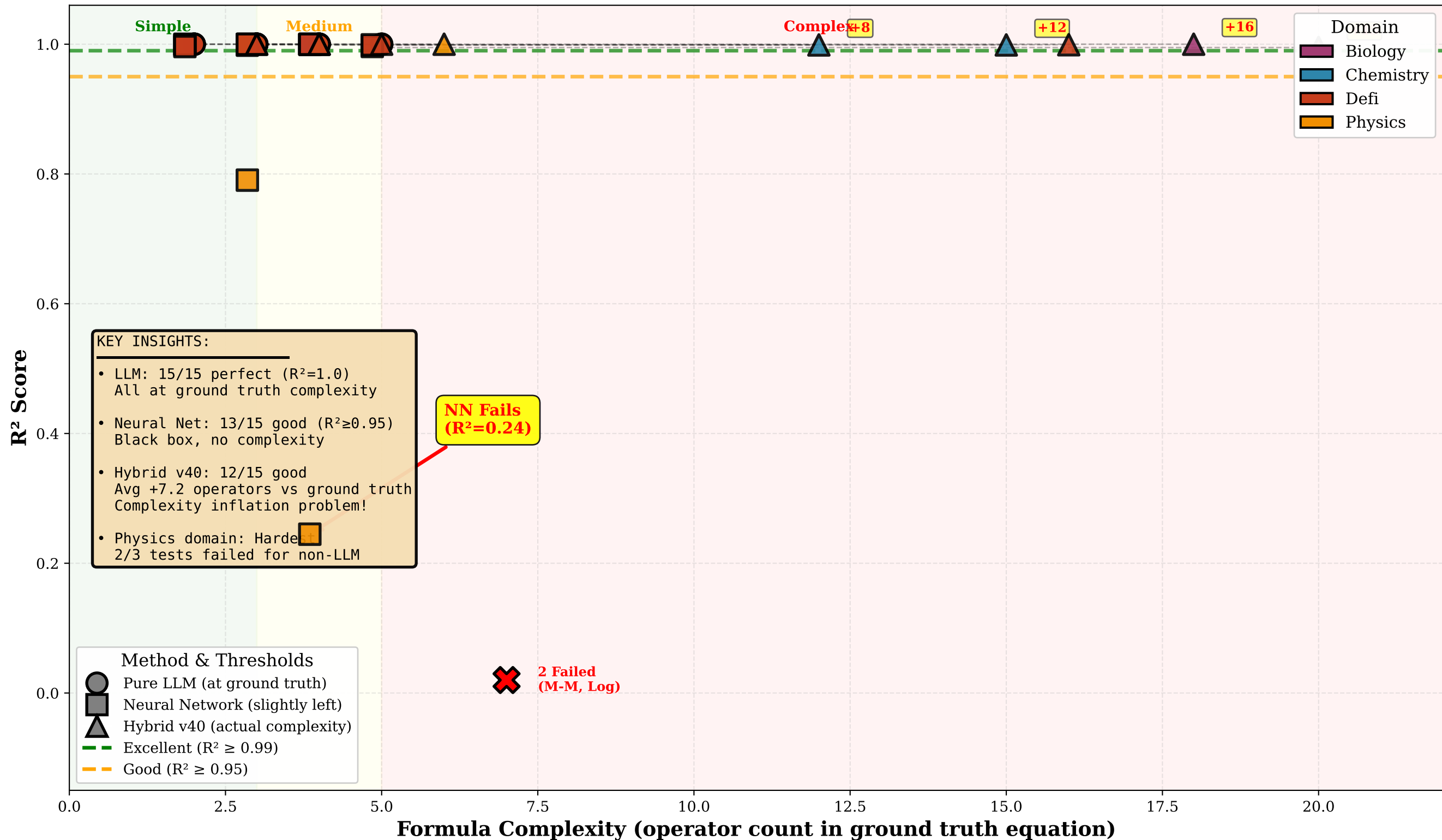
Figure 4: Accuracy vs Complexity Trade-off Pure LLM at Ground Truth | Hybrid v40 Shows Complexity Inflation
