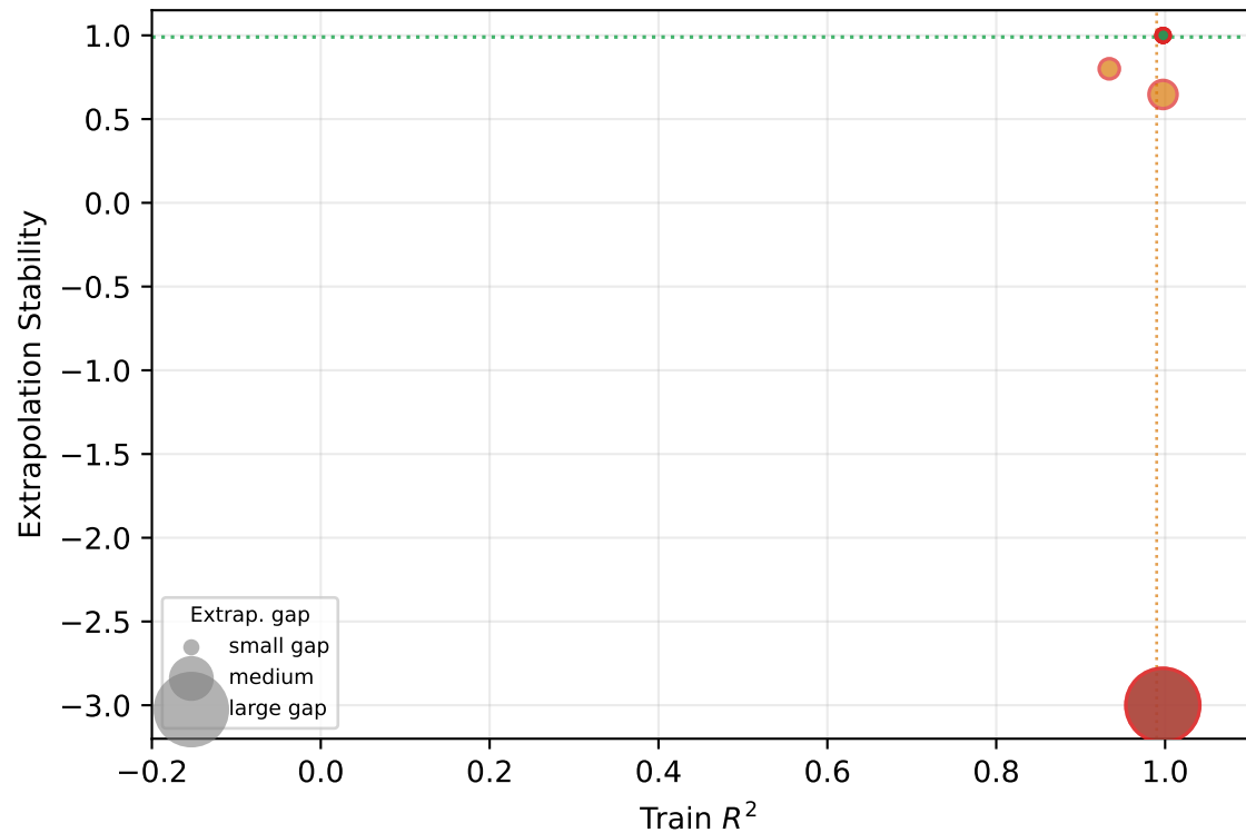
Neural Net
