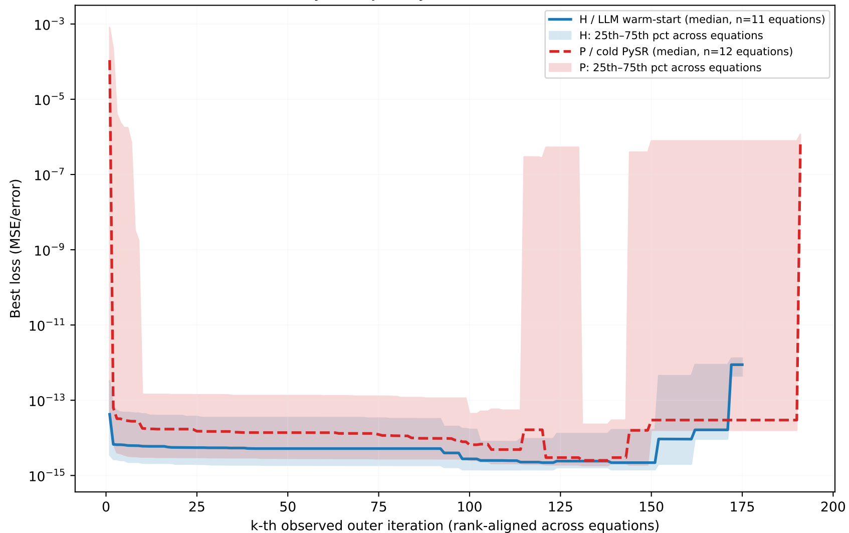
PySR trajectory overview — seed 123
