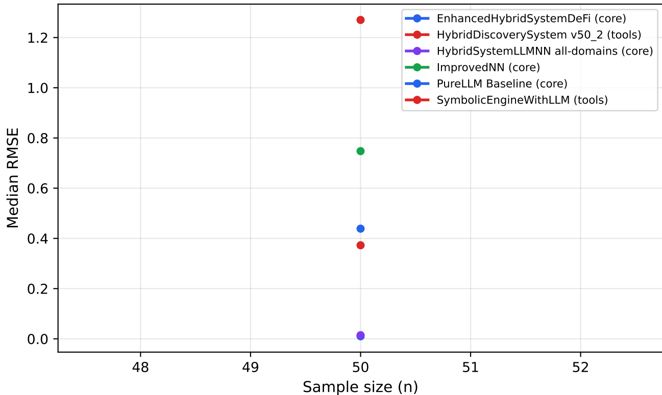
Median RMSE vs Sample Size
