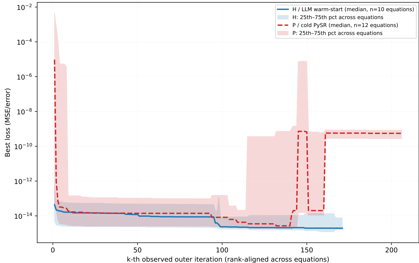
PySR trajectory overview — seed 42
