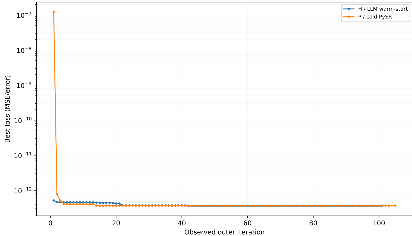
Nguyen N3 — seed 777
