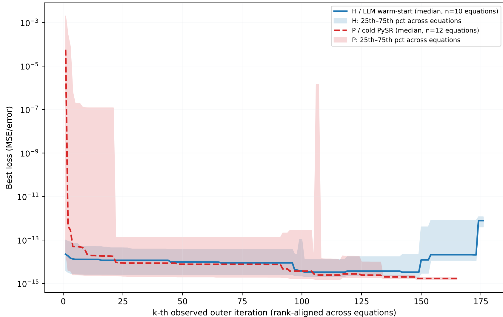
PySR trajectory overview — seed 777
