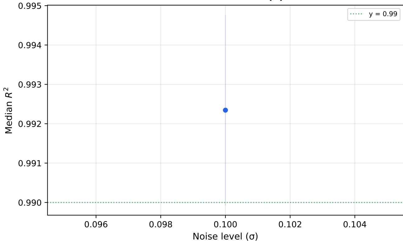
Median R^2 vs Noise ( \sigma )
