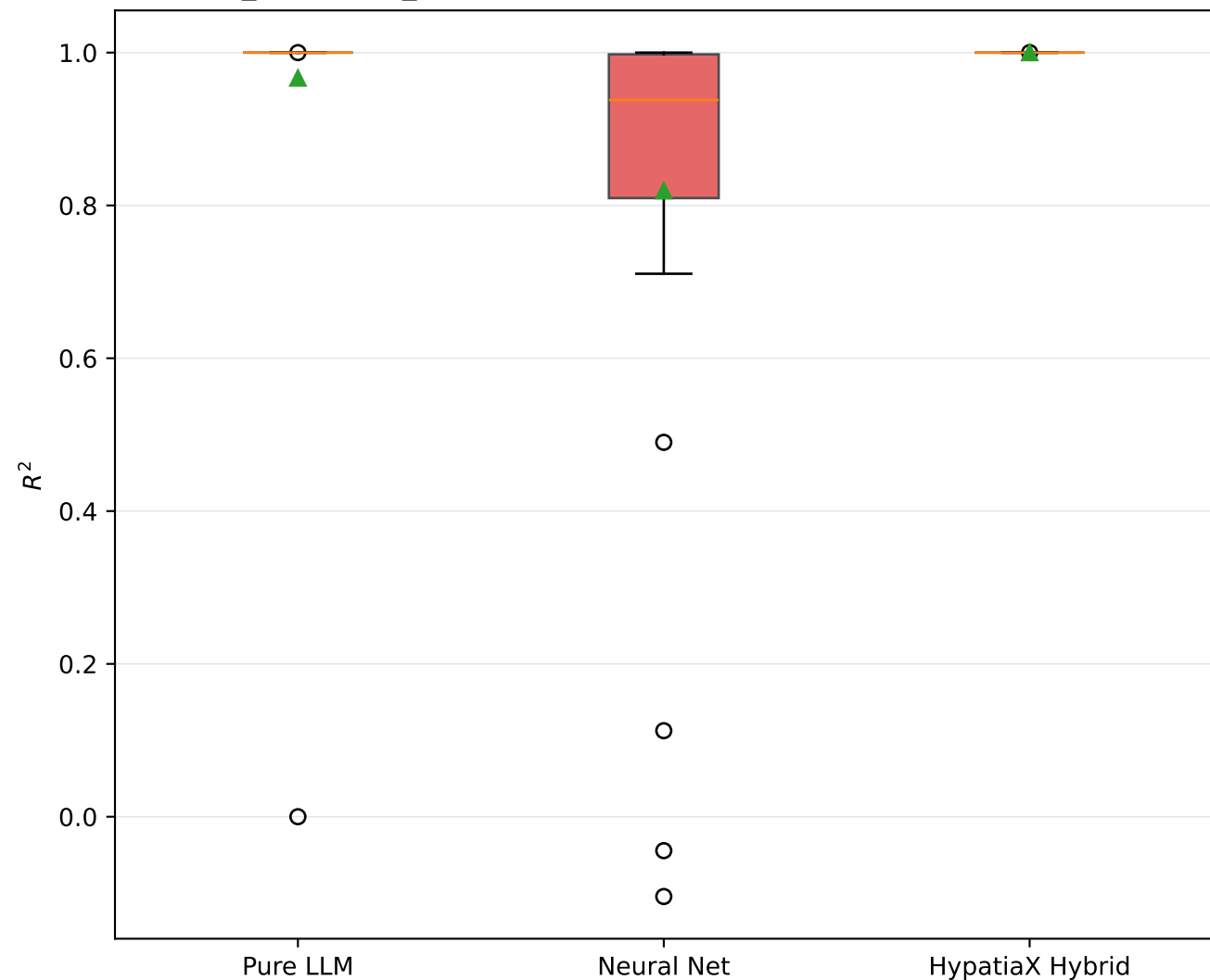
exp2_feynman_pca — R^2 by System (Pure LLM / NN / Hybrid)
