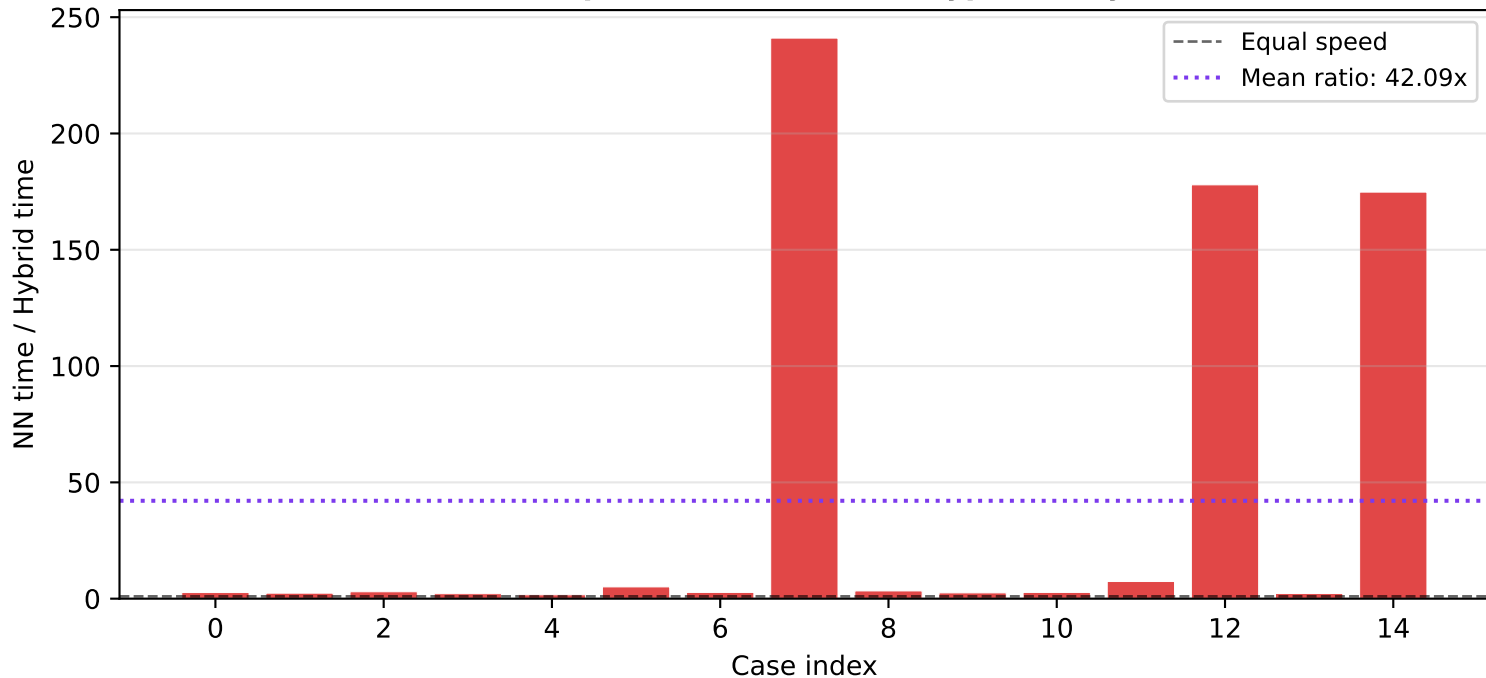
Relative Speed: Neural Net vs HypatiaX Hybrid
