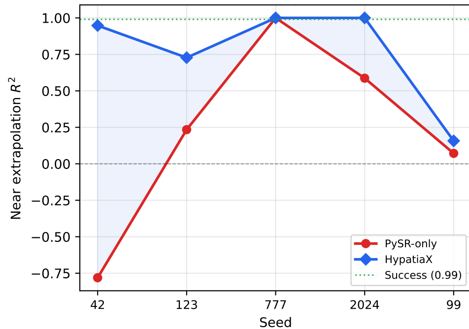
Near Extrapolation
