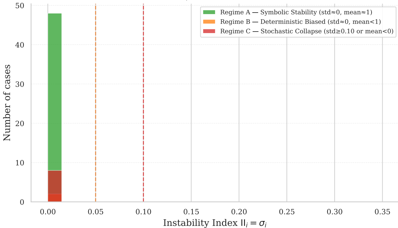
Distribution of LLM Instability Index \Pi_i = \sigma_i = \text{std}(R_i^2) across independent runs
