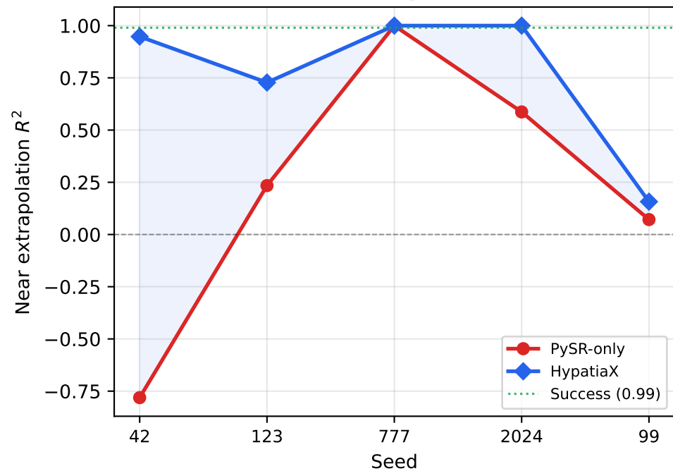
Near Extrapolation
