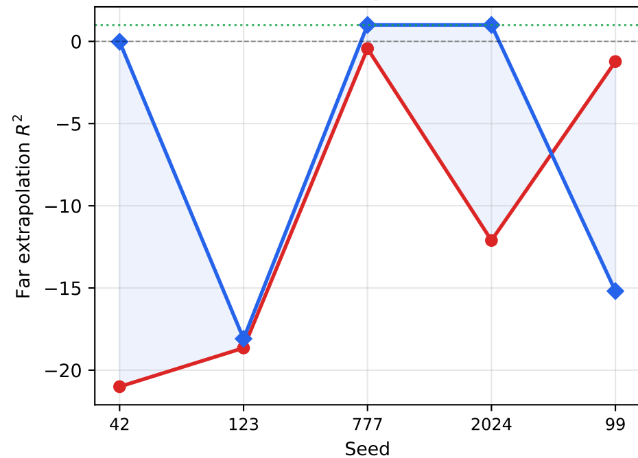
Far Extrapolation
