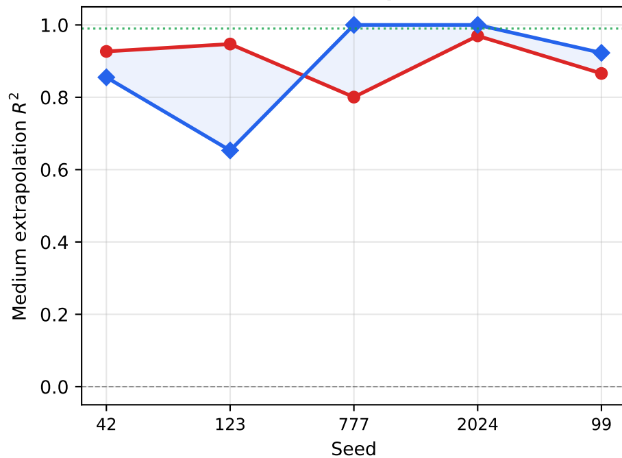
Medium Extrapolation
