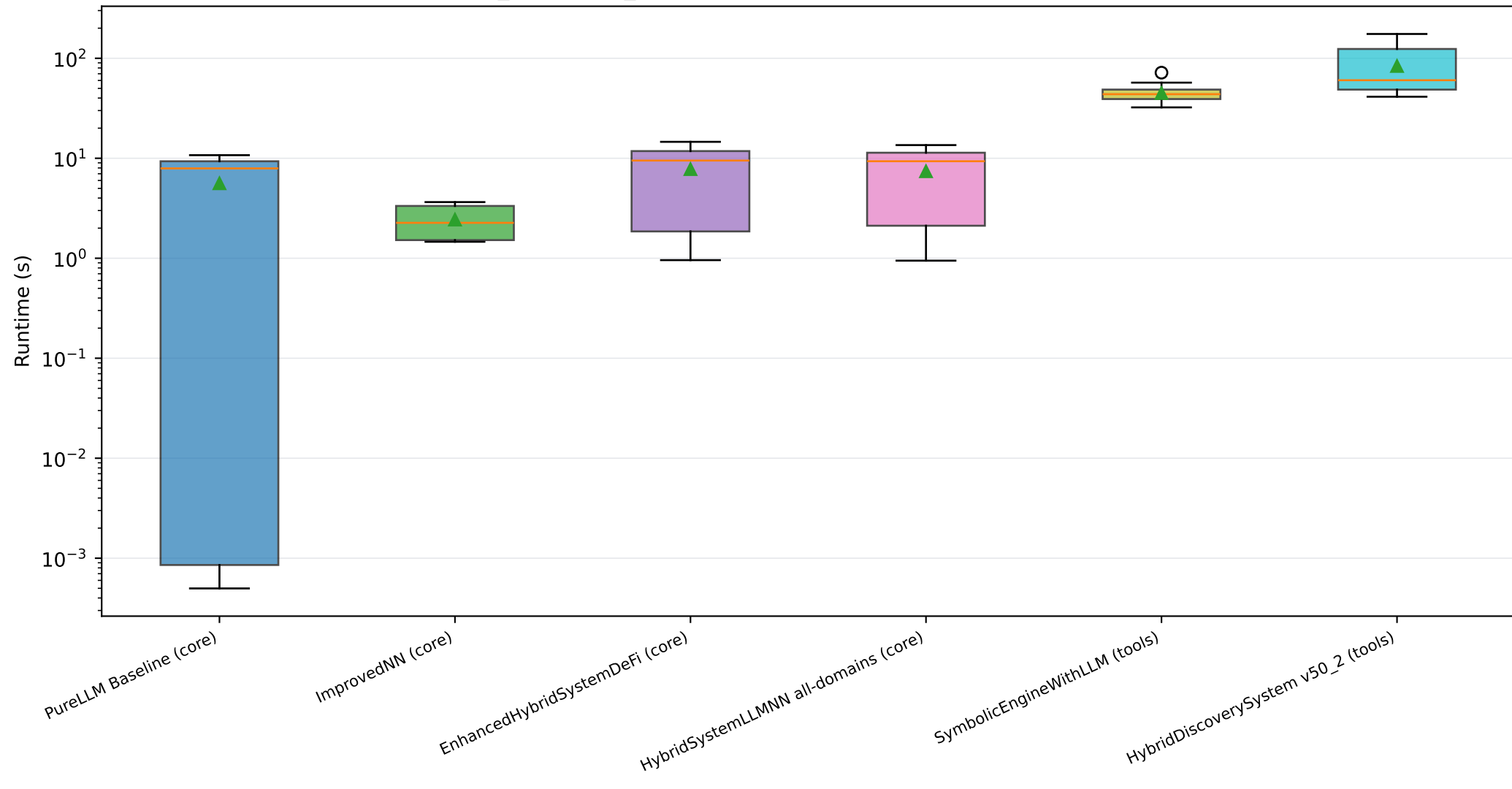
exp2_feynman_pca — Runtime by Method (all 6 systems)
