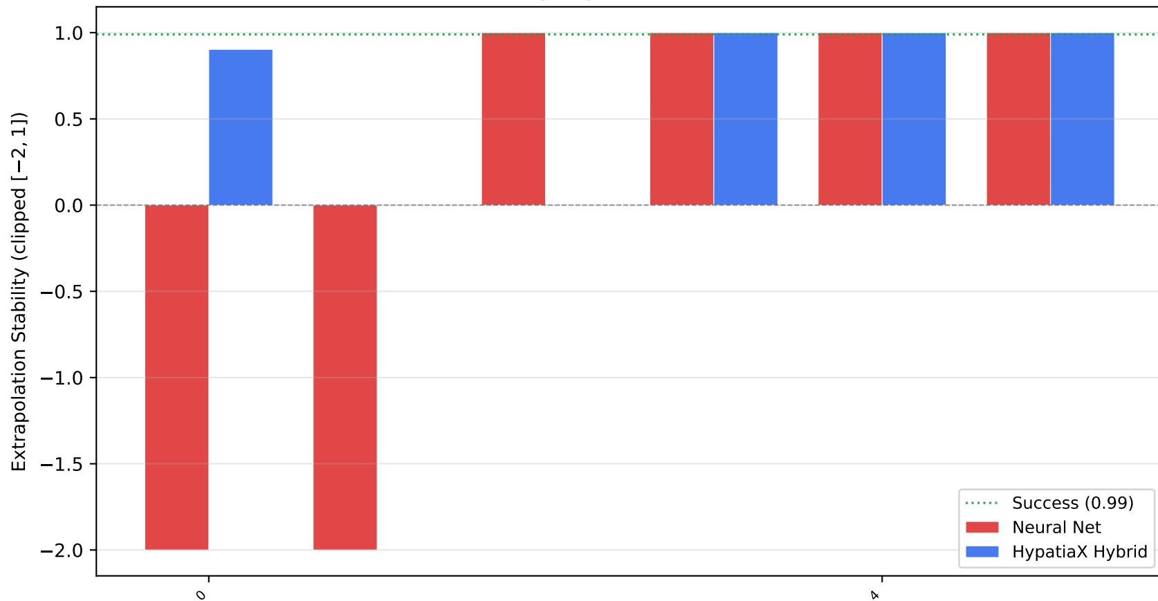
Extrapolation Stability: HypatiaX vs Neural Net (All Cases)
