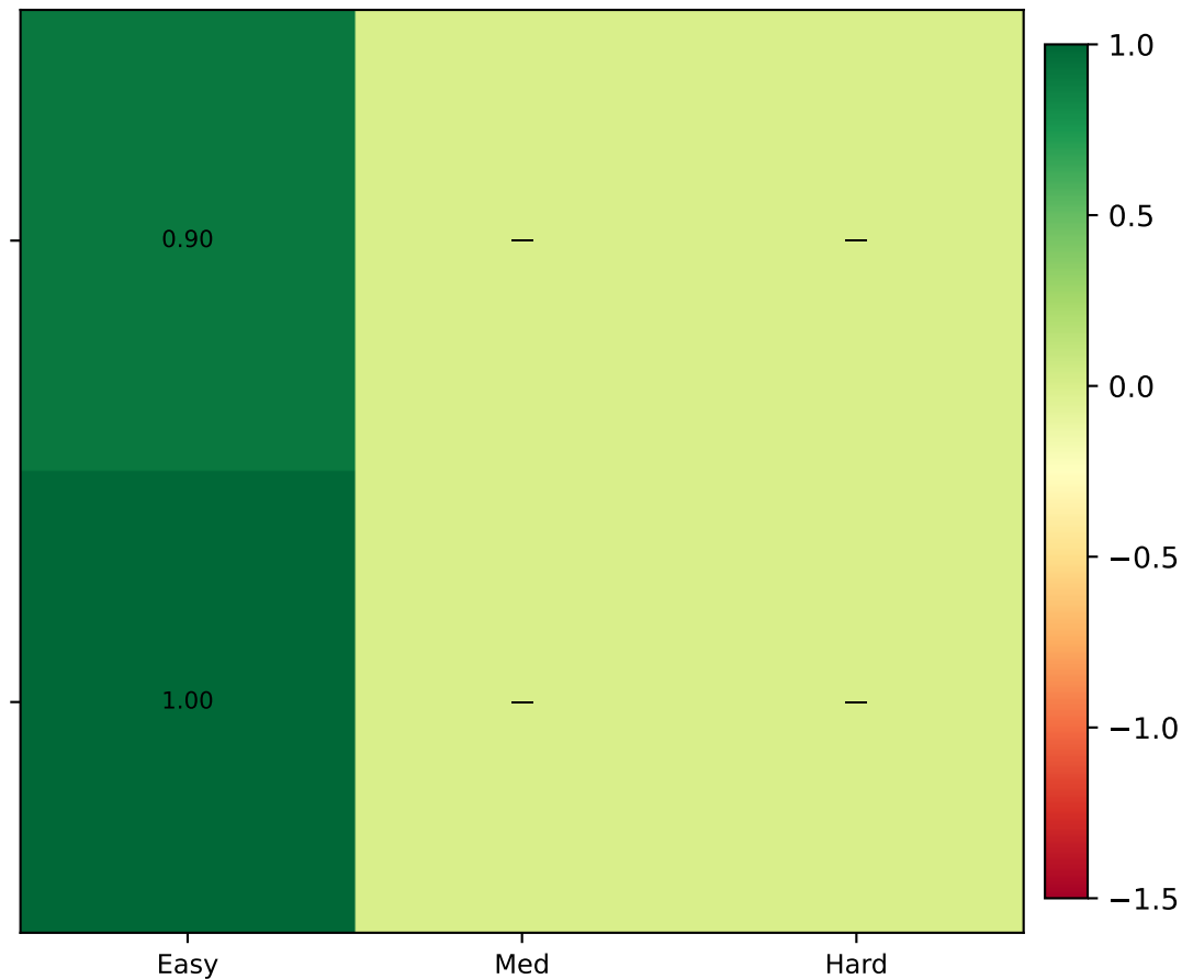
HypatiaX Hybrid
