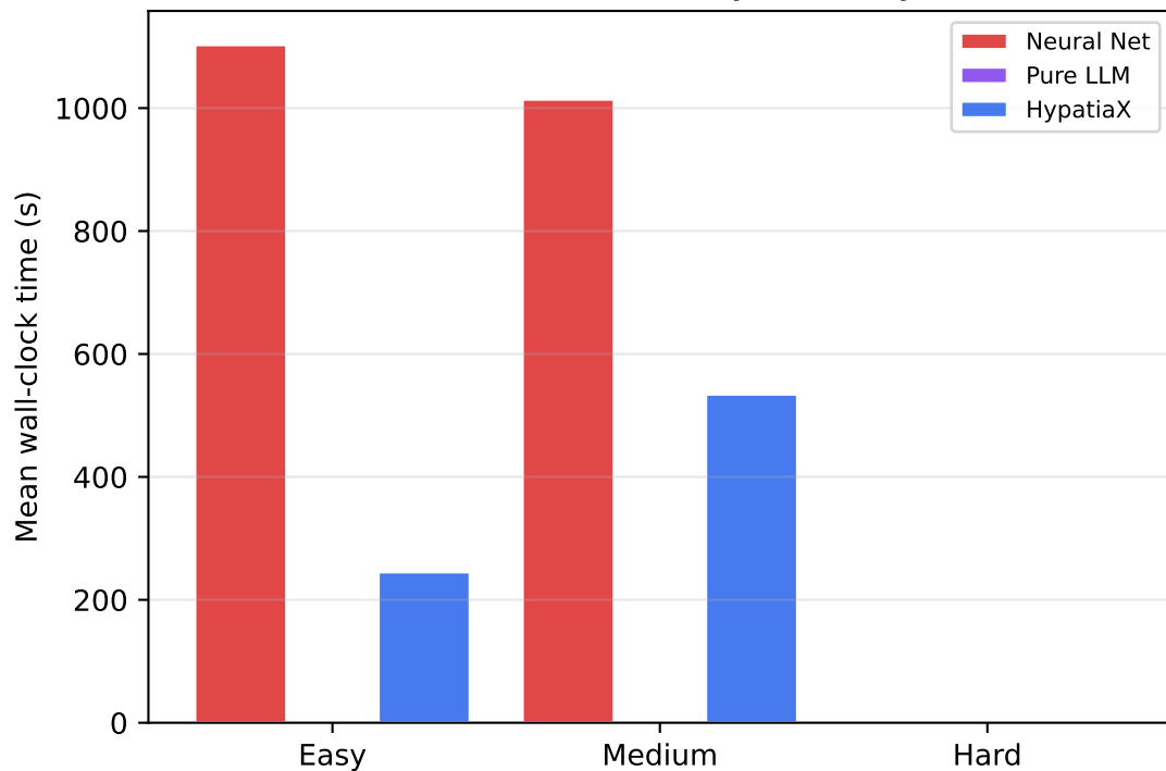
Mean Solve Time by Difficulty
