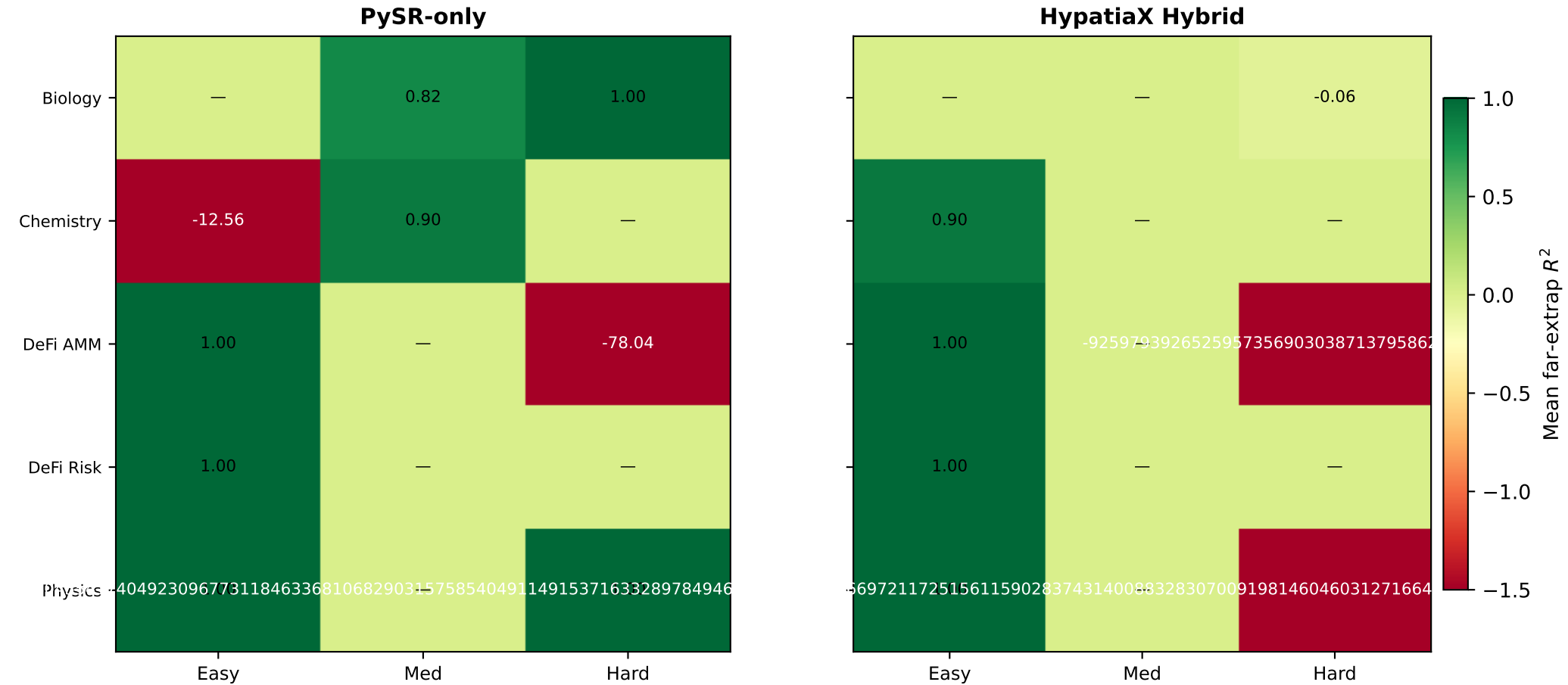
Far-Extrap R^2 : PySR-only vs HypatiaX (Formula Type \times Difficulty)
