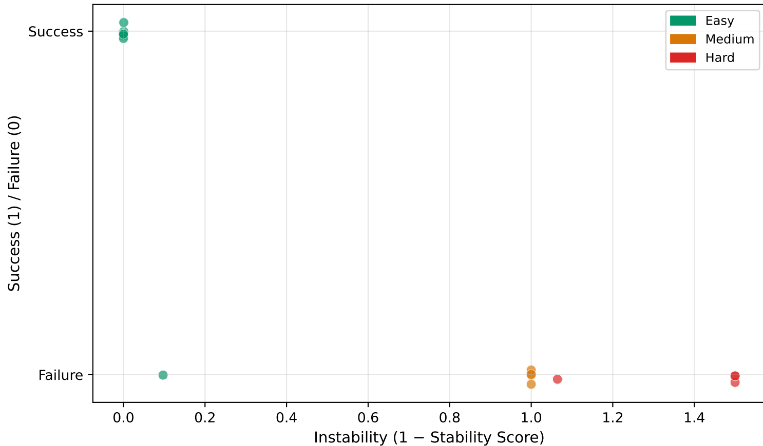
Success vs Instability (HypatiaX Hybrid)
