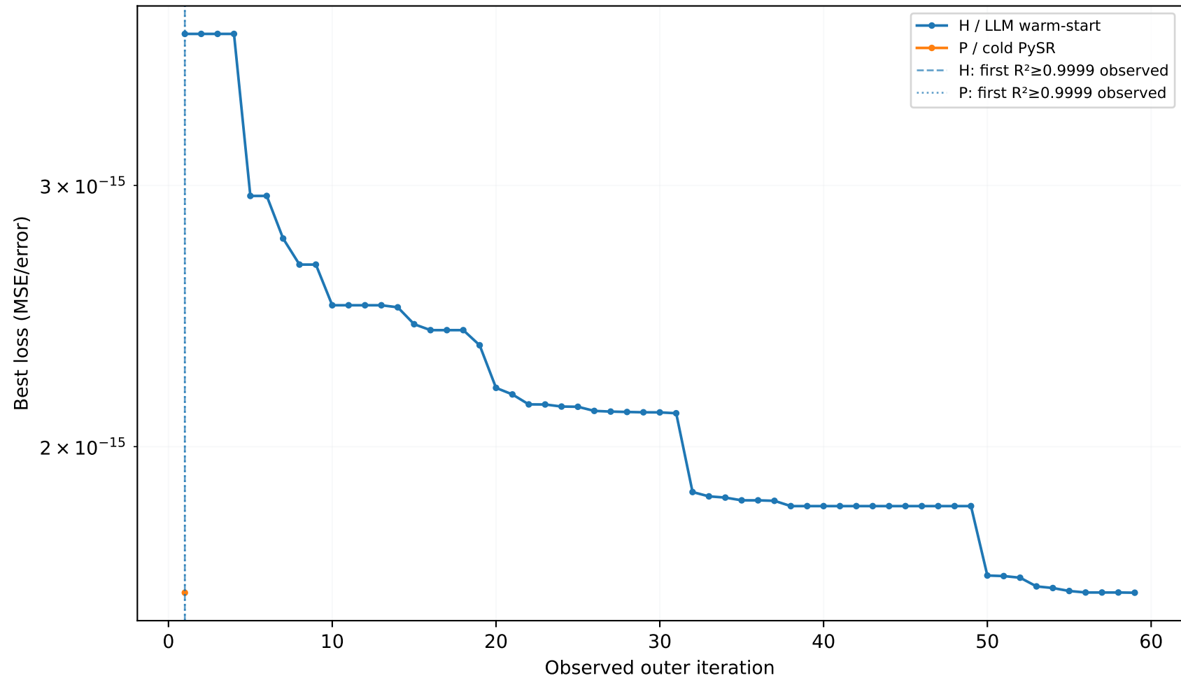
Nguyen N1 — seed 99
