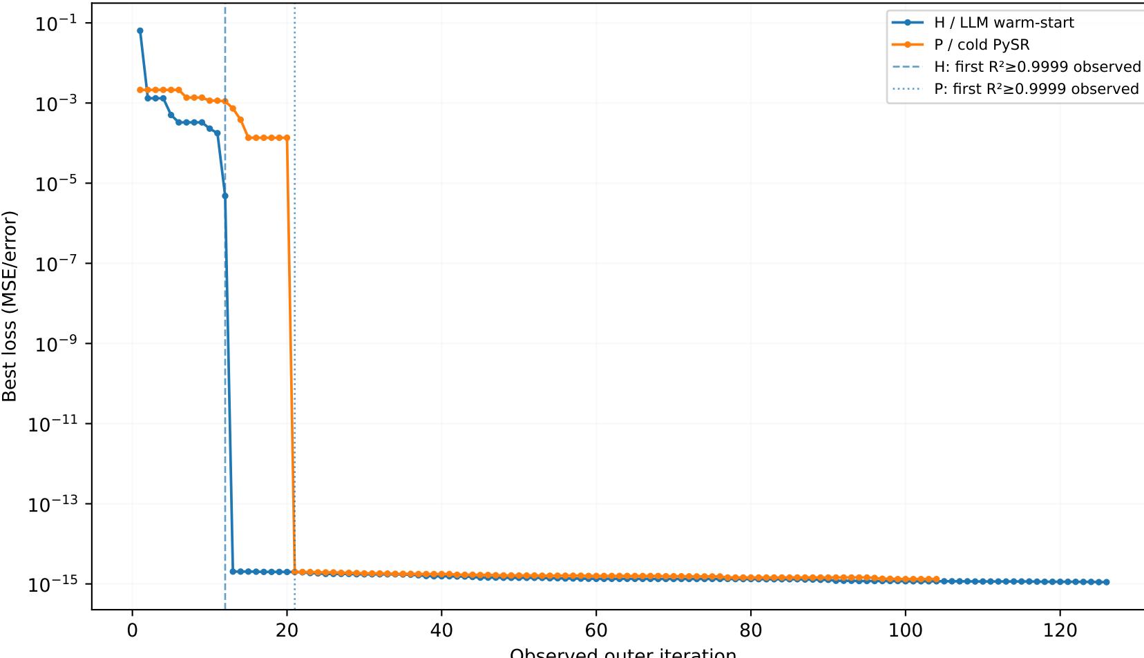
Nguyen N10 — seed 99
