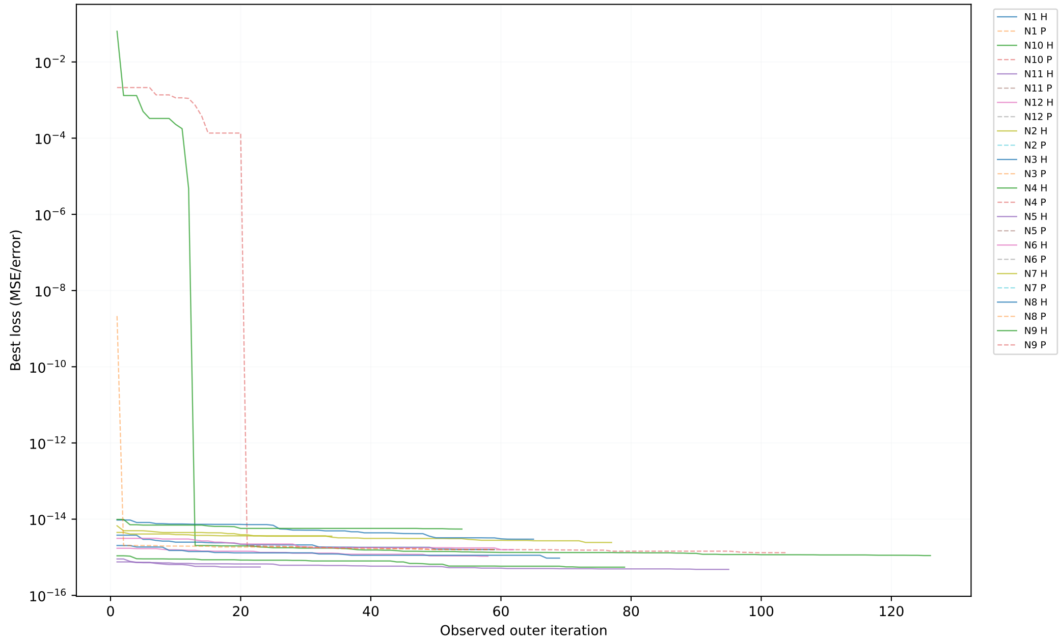
PySR trajectory overview — seed 99
