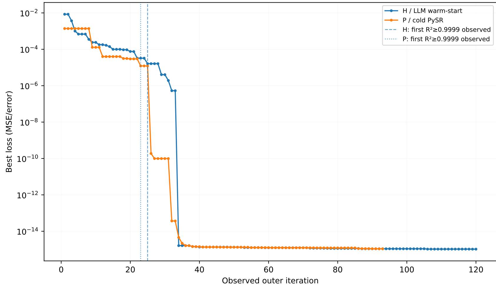
Nguyen N10 — seed 2024
