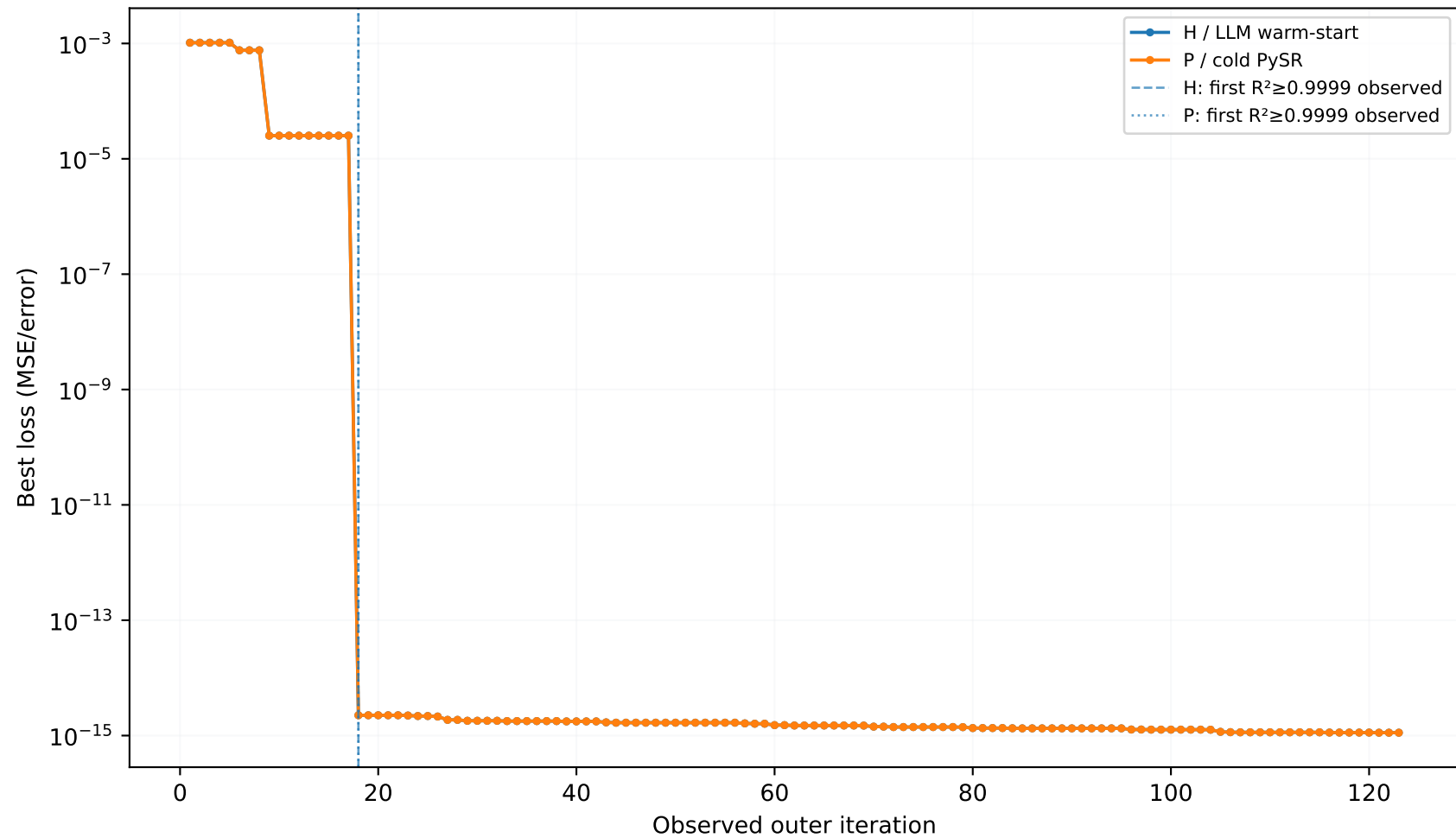
Nguyen N10 — seed 42
