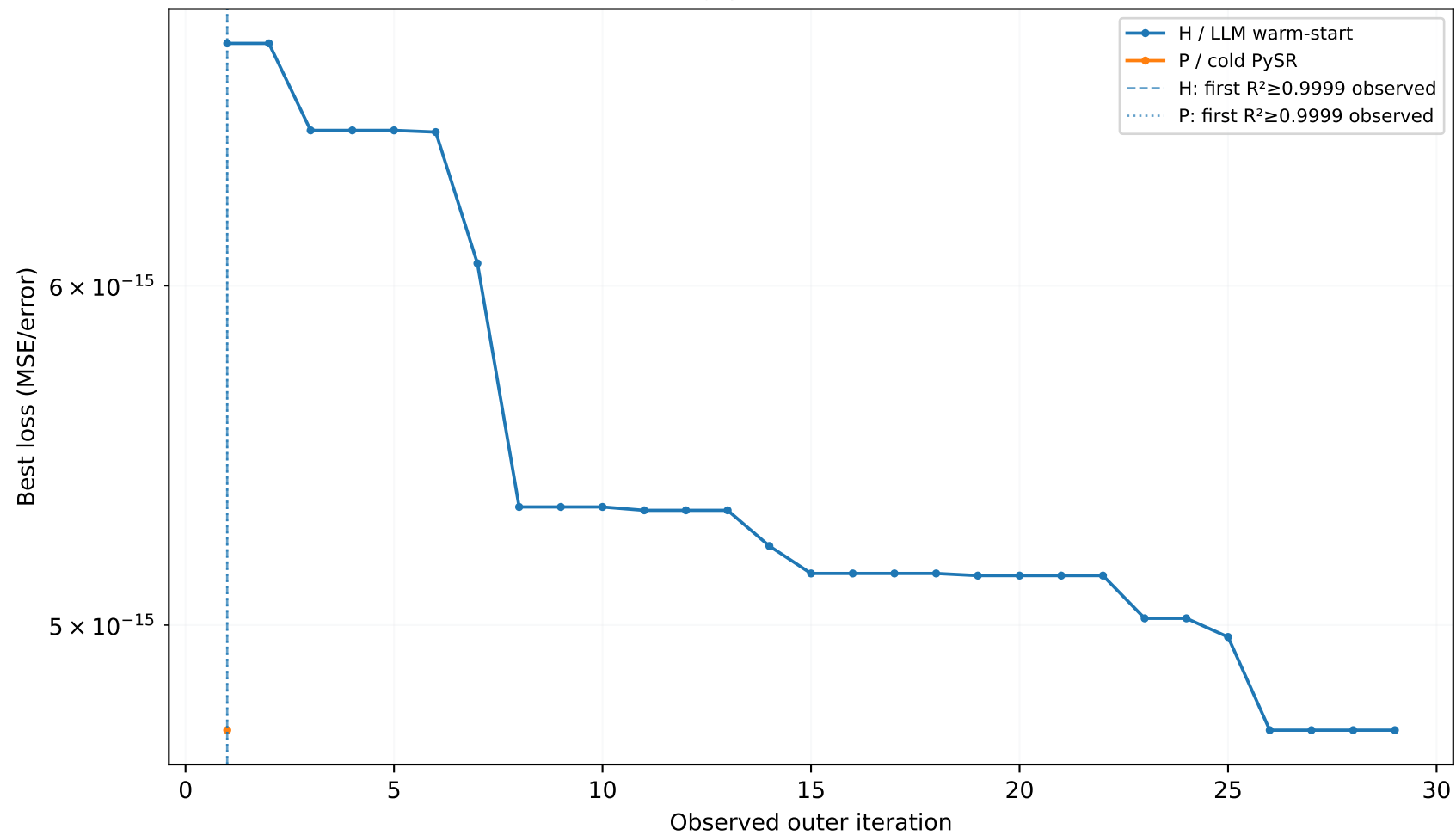
Nguyen N2 — seed 42
