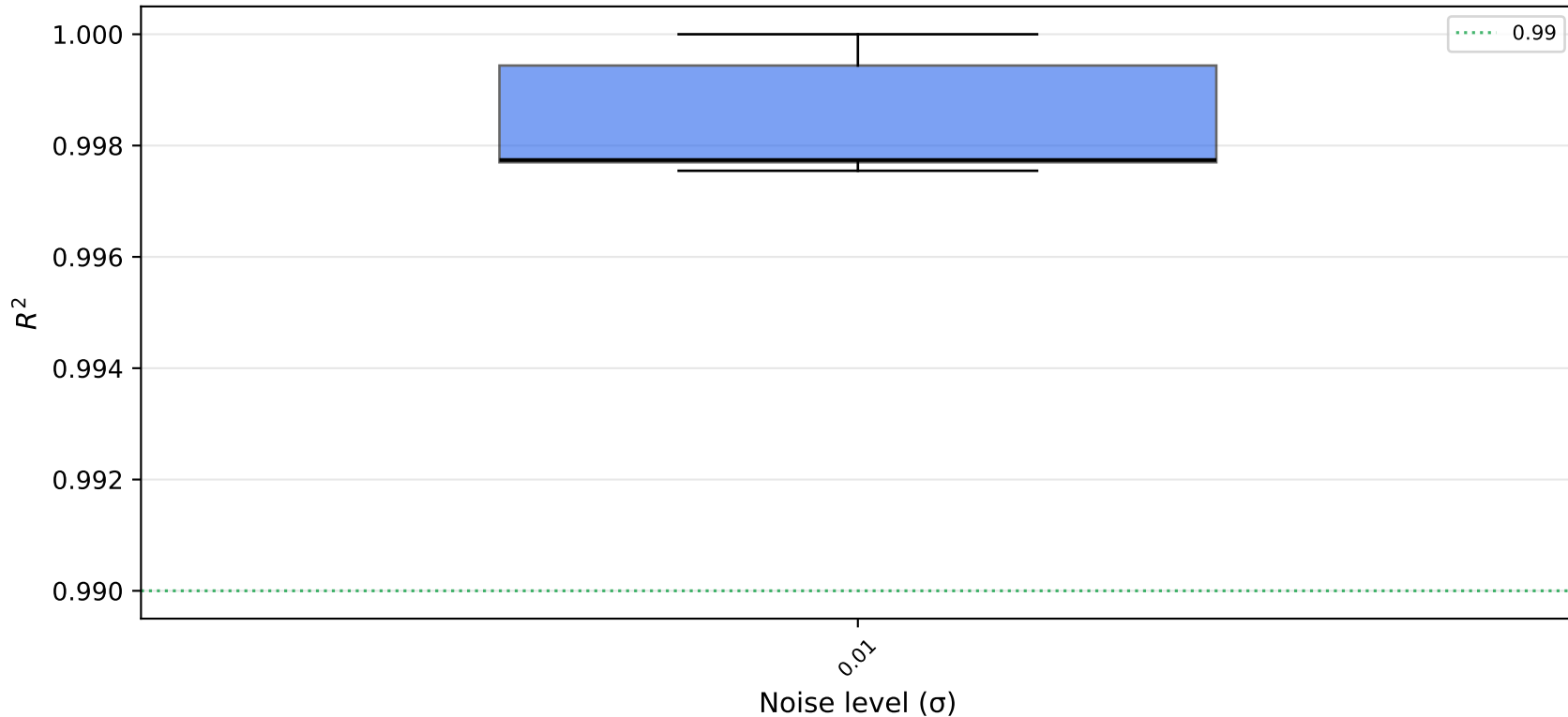
Per-Equation R^2 Box Plots vs Noise ( \sigma )
