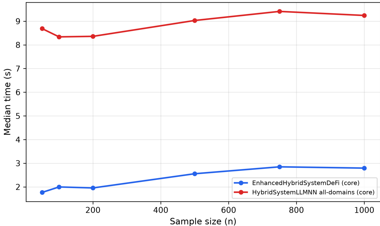
Median Solve Time vs Sample Size
