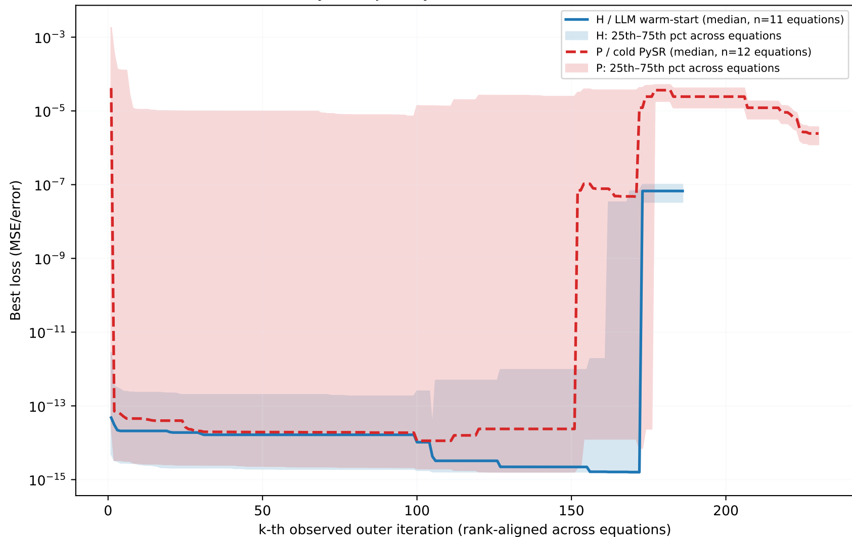
PySR trajectory overview — seed 2024
