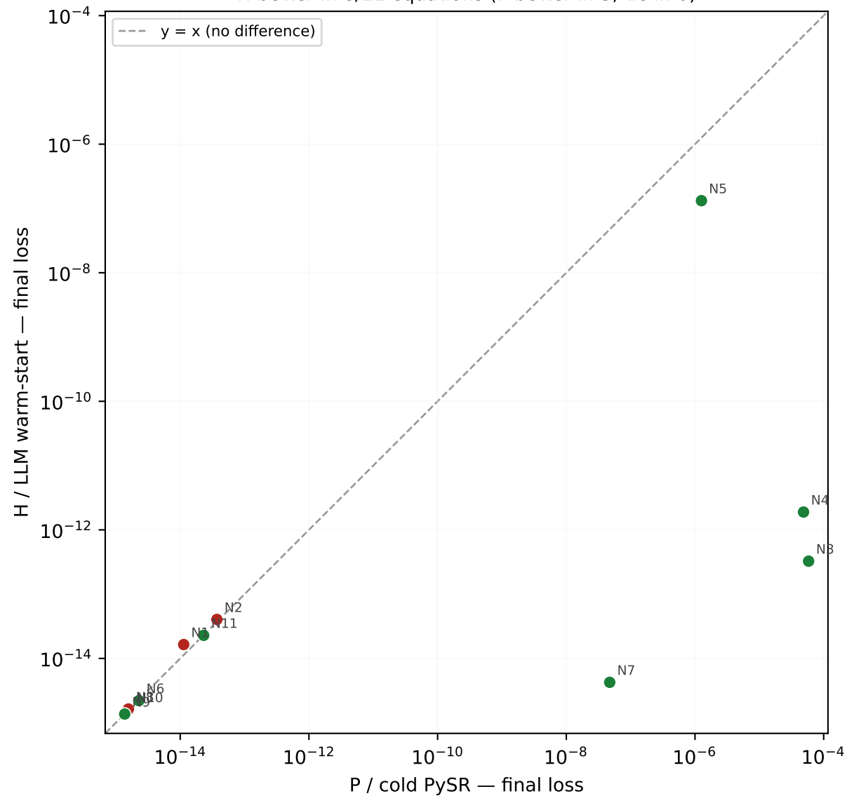
Final-loss win/loss — seed 2024 H better in 8/11 equations (P better in 3, tie in 0)
