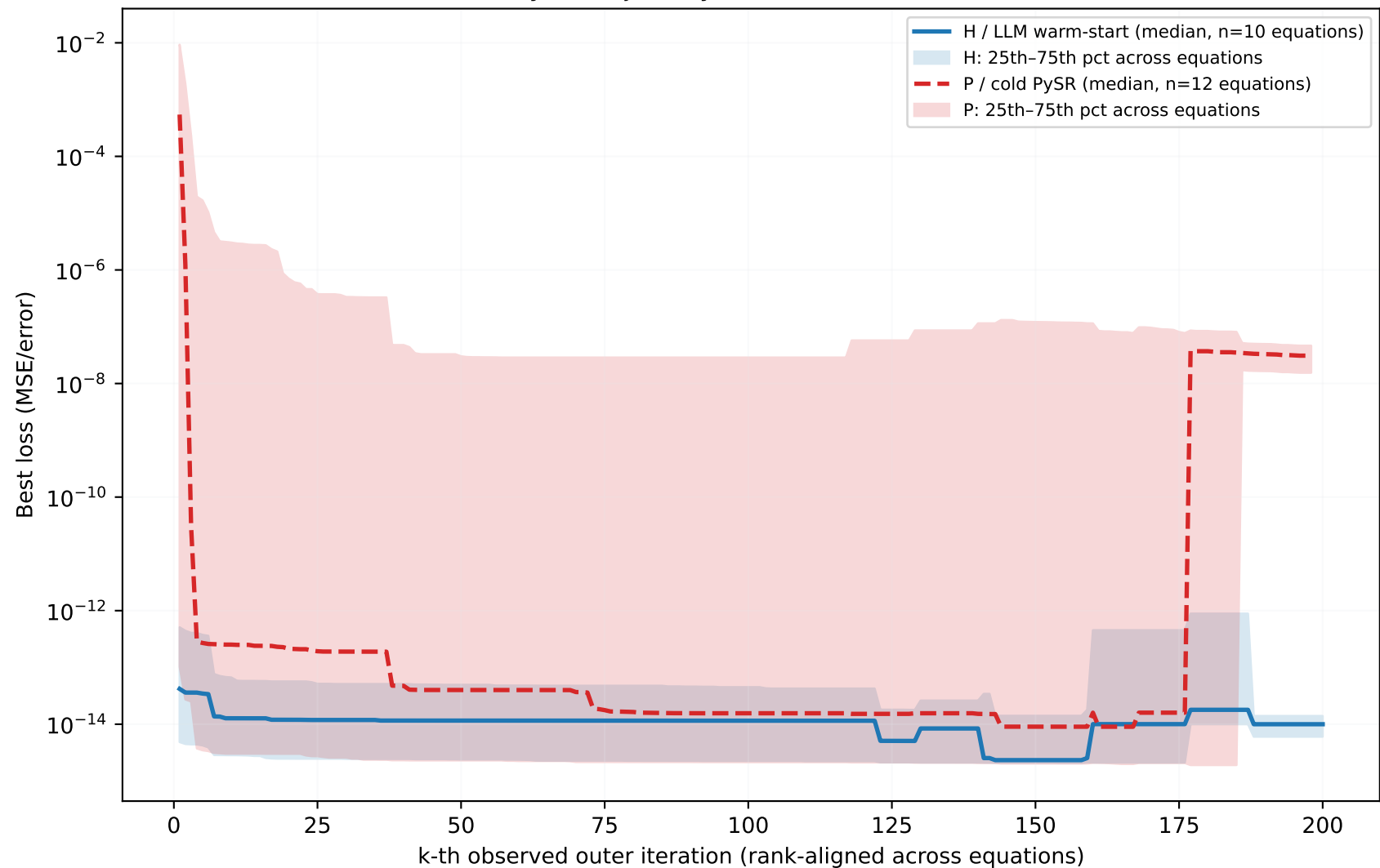
PySR trajectory overview — seed 99
