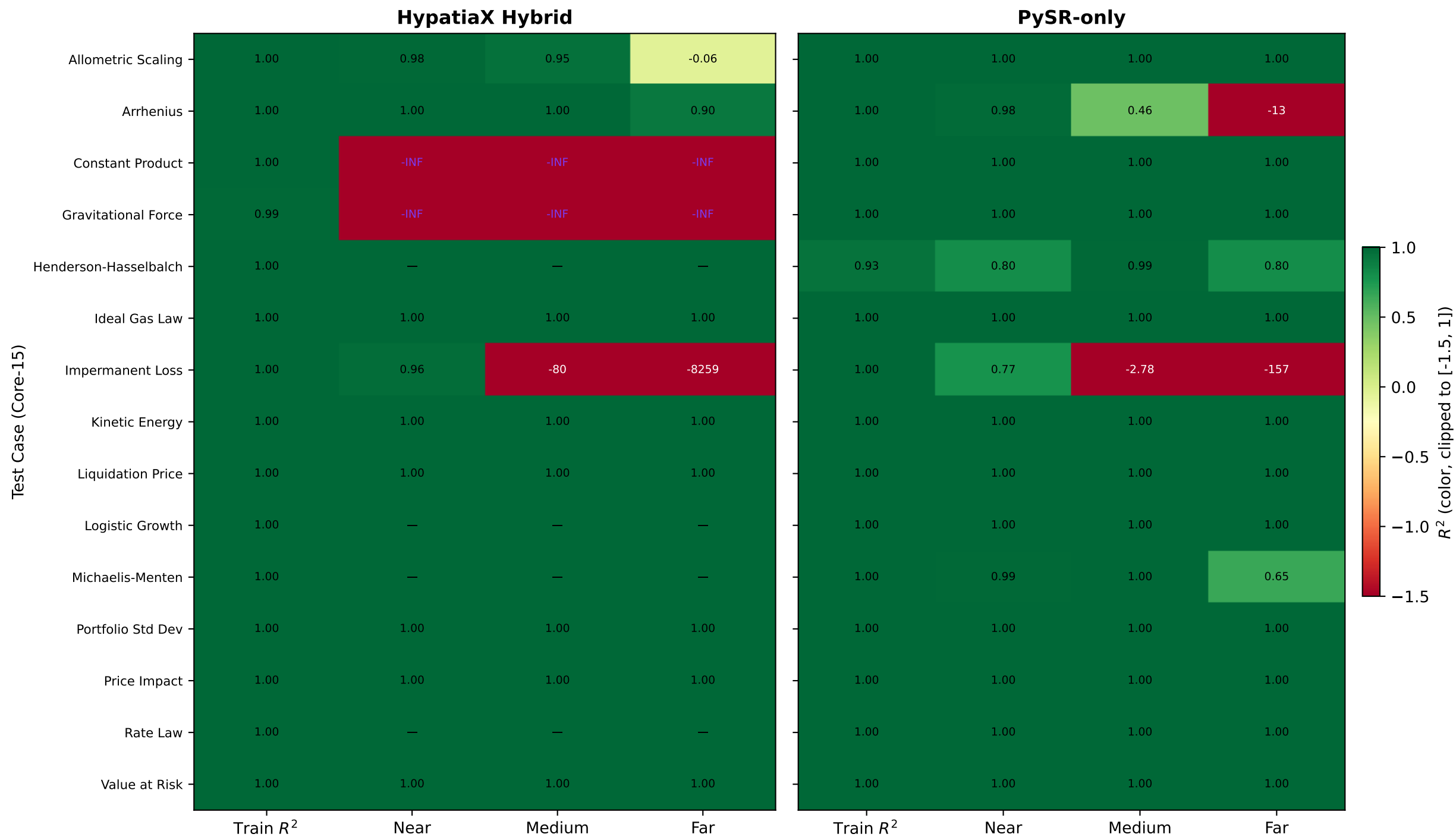
Figure 4 (regenerated): R^2 Heatmap — Raw (unclipped) values, Train/Near/Medium/Far
