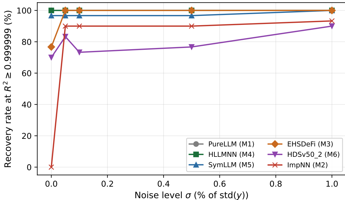
Recovery rate vs. noise level (July 2026 rerun, n = 200 , 30 equations)
