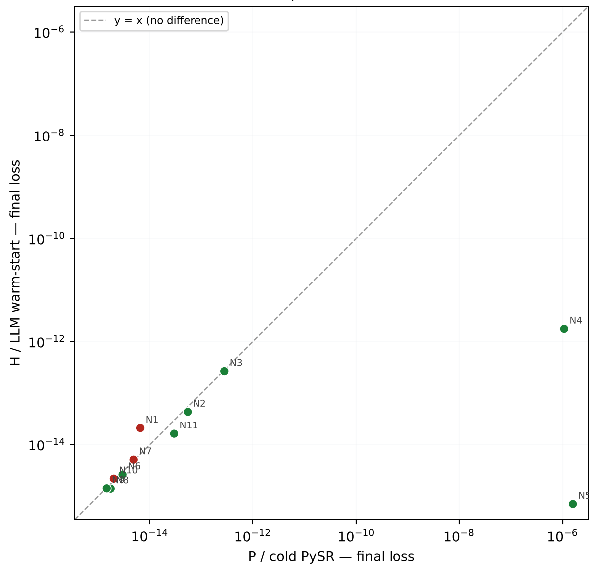
Final-loss win/loss — seed 123 H better in 8/11 equations (P better in 3, tie in 0)
