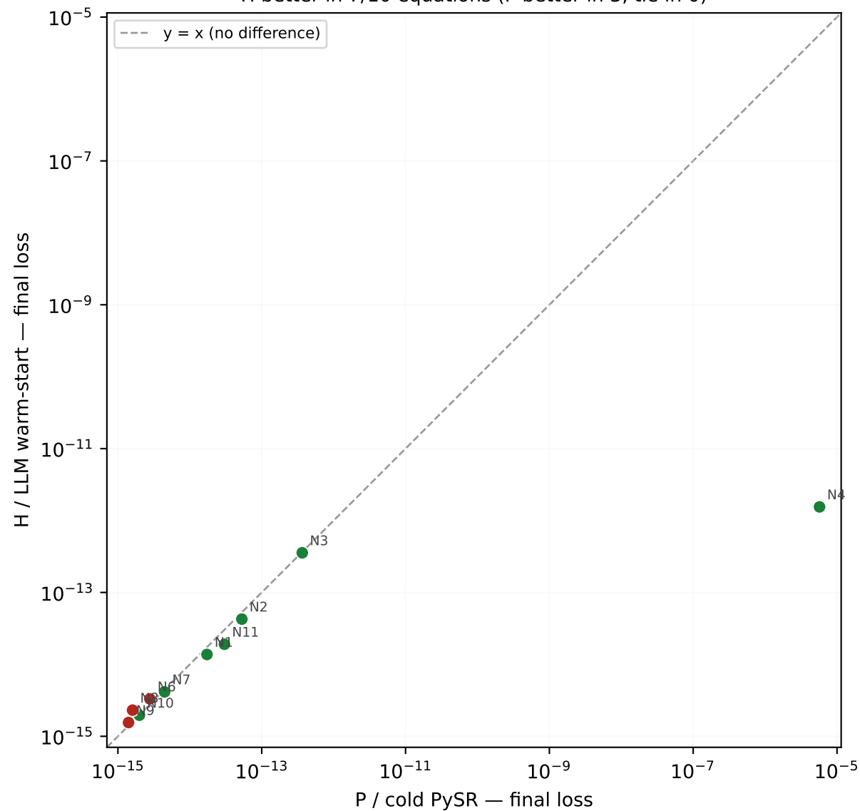
Final-loss win/loss — seed 777 H better in 7/10 equations (P better in 3, tie in 0)
