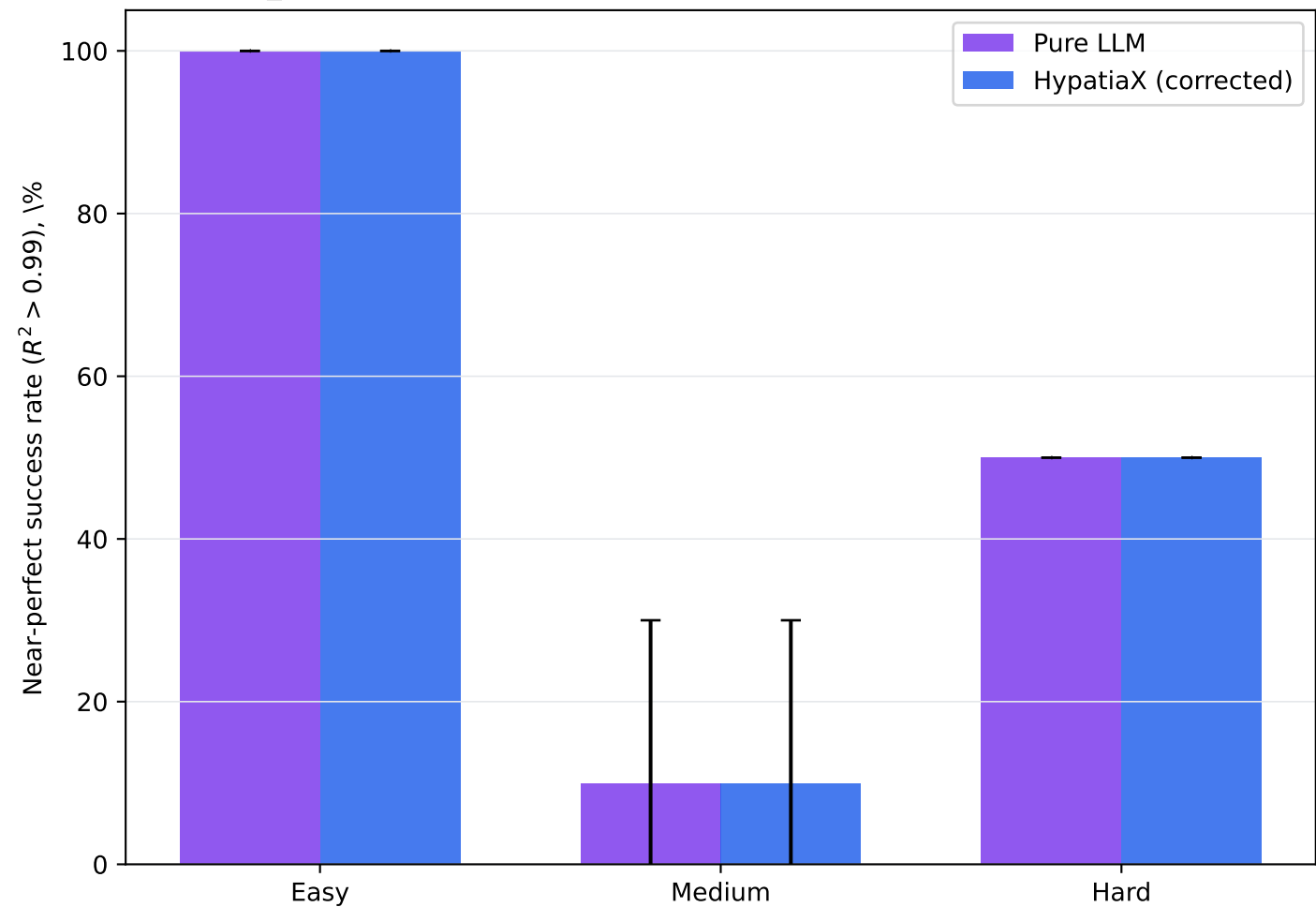
exp1b_pca — Noise-robust DeFi benchmark (5 seeds, mean \pm std)
