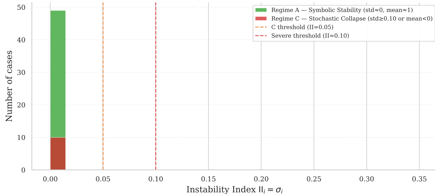
Distribution of Instability Index across Benchmark Cases
