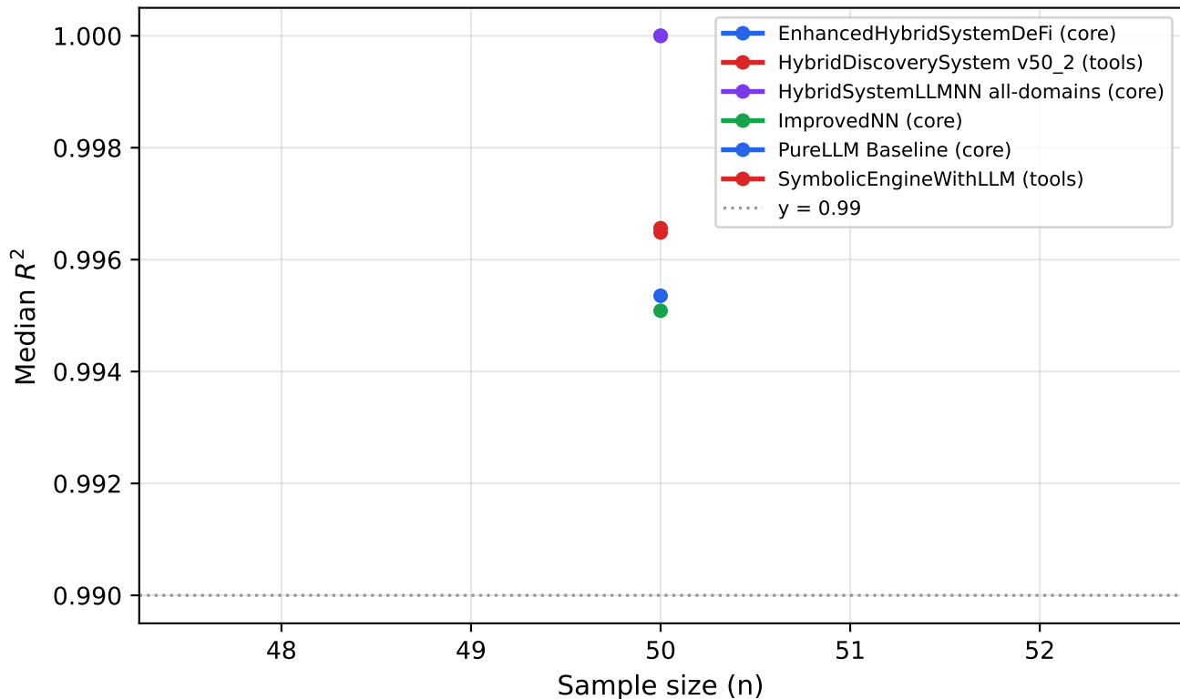
Median R^2 vs Sample Size
