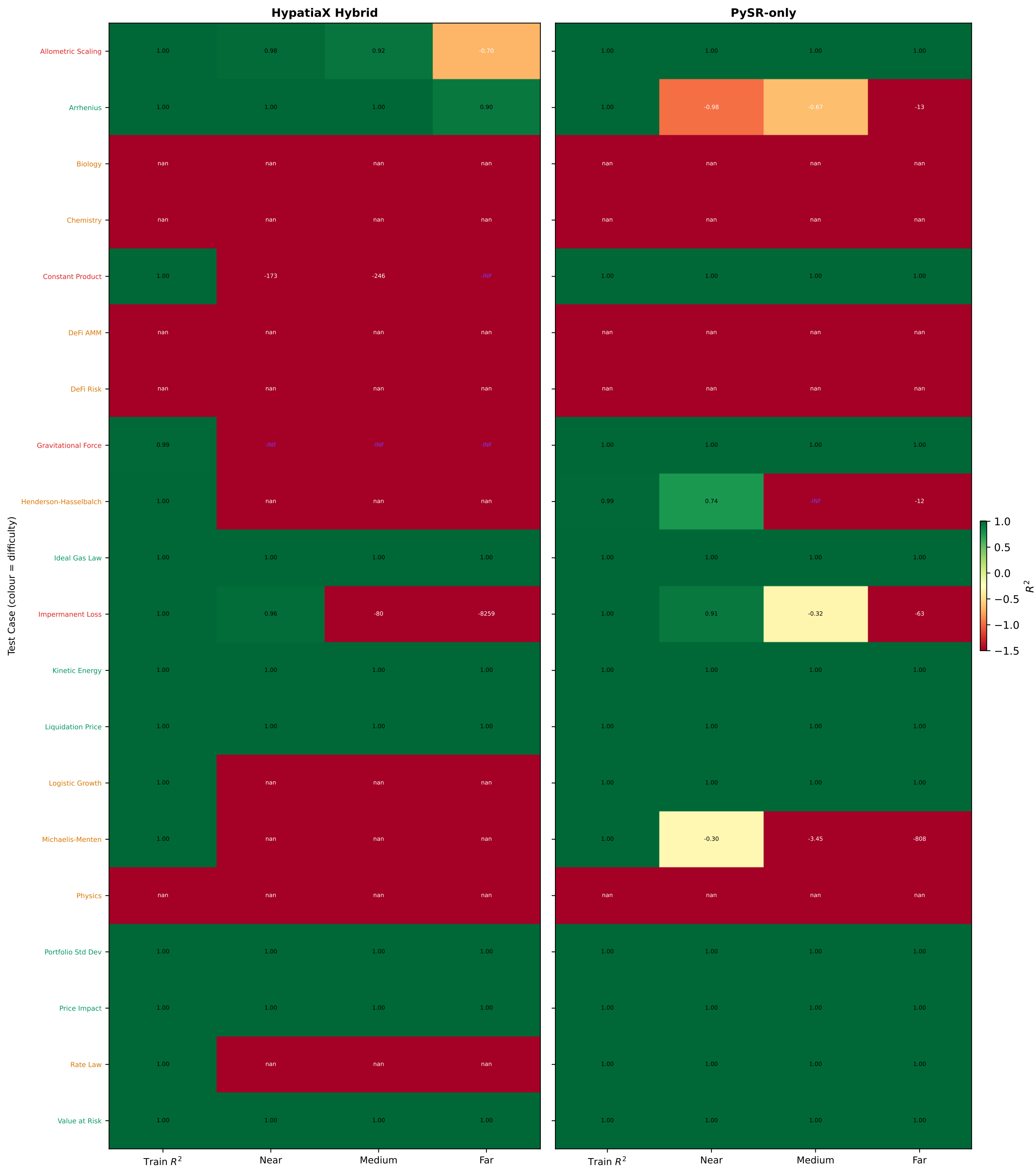
R^2 Heatmap: Train / Near / Medium / Far Regimes
