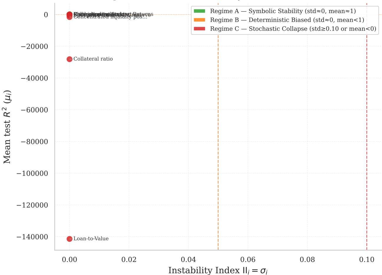
Mean R^2 vs Instability Index LLMs operate in two distinct modes: Symbolic (A) vs Stochastic (C)
