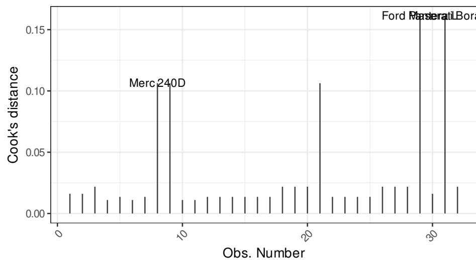
Cook's distance
