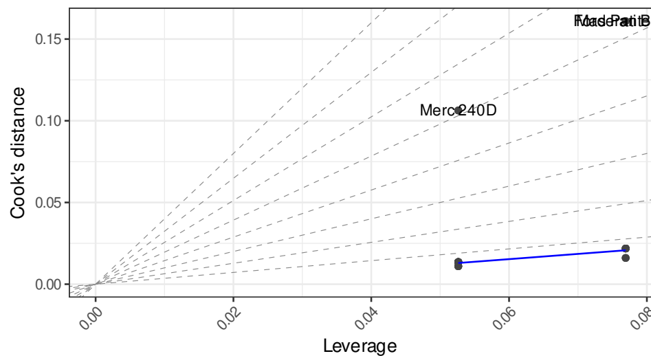
Cook's dist vs Leverage
