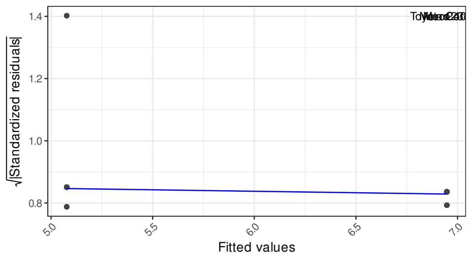
Scale-Location
