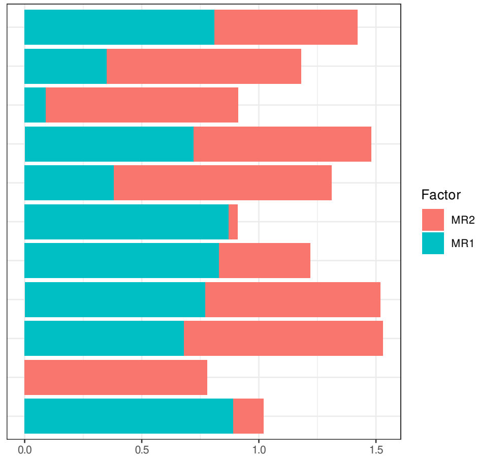
Structure Matrix Loadings
