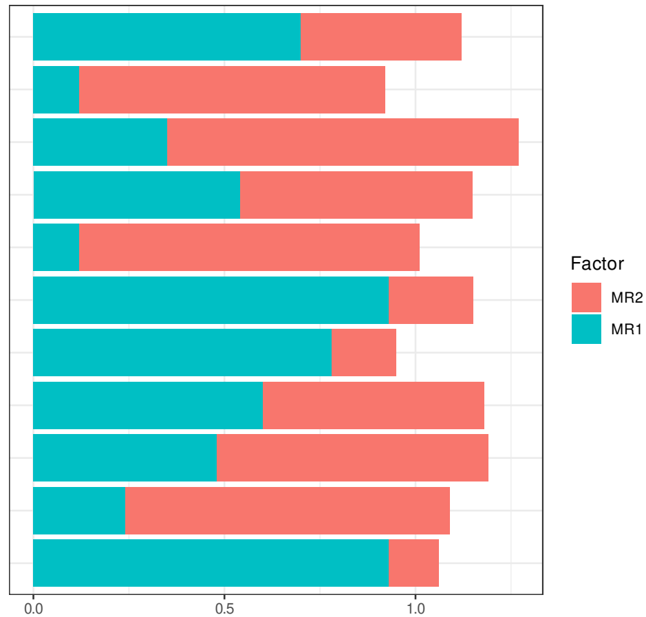
Pattern Matrix Loadings
