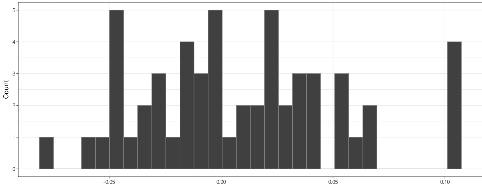
Histogram of residuals
