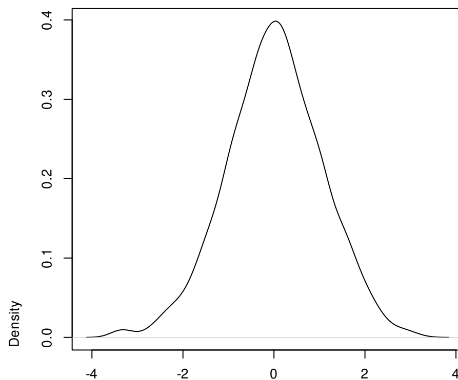
Density Function
