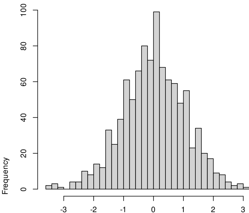
Histogram
