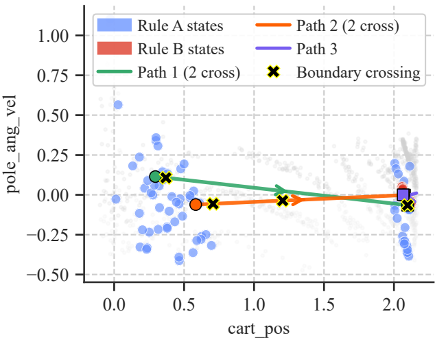
CartPole: mergeable pair (sim=0.70, crossing rate=87%)
