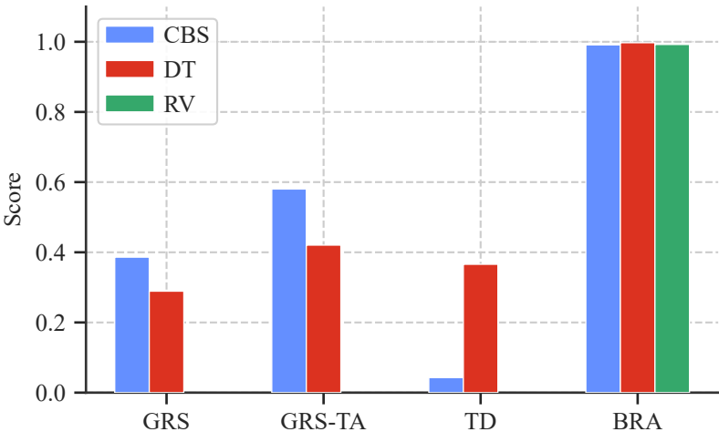
MiniGrid-Dynamic-Obstacles-8x8-v0 (PPO)
