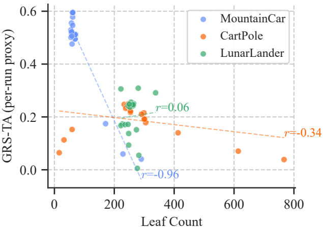
Tree Complexity vs. Structural Stability
