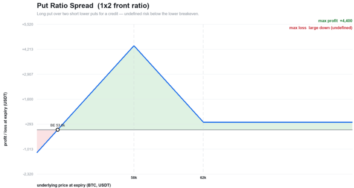
Put ratio spread payoff
