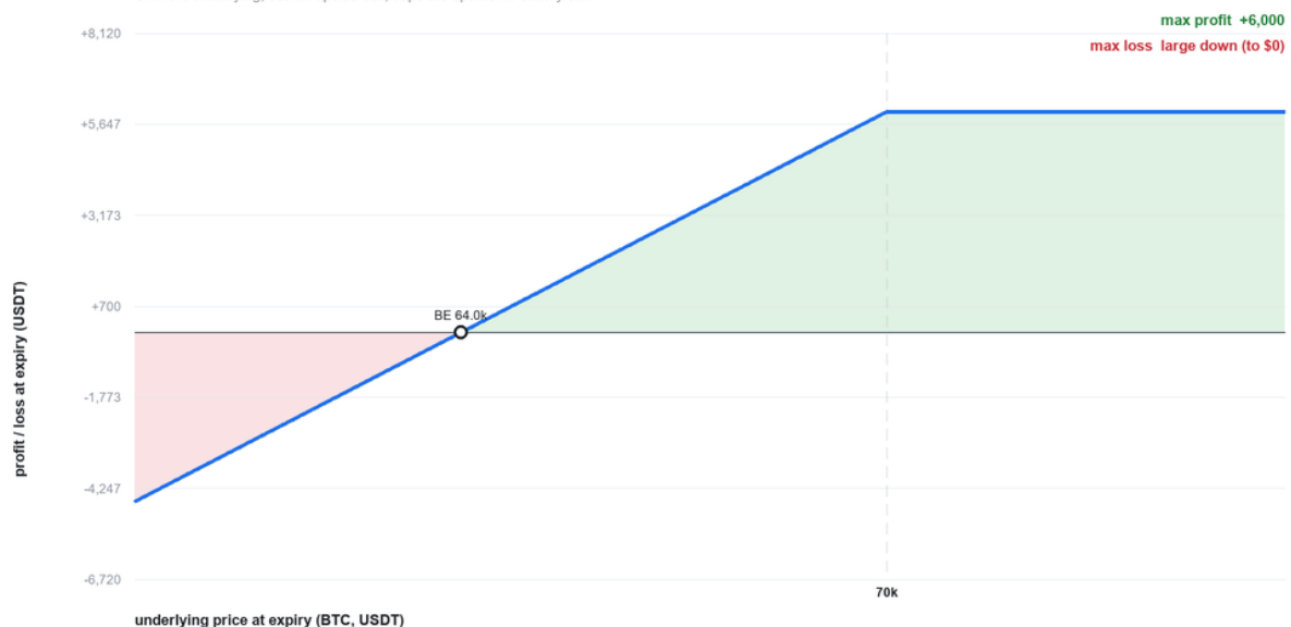
Covered call payoff
