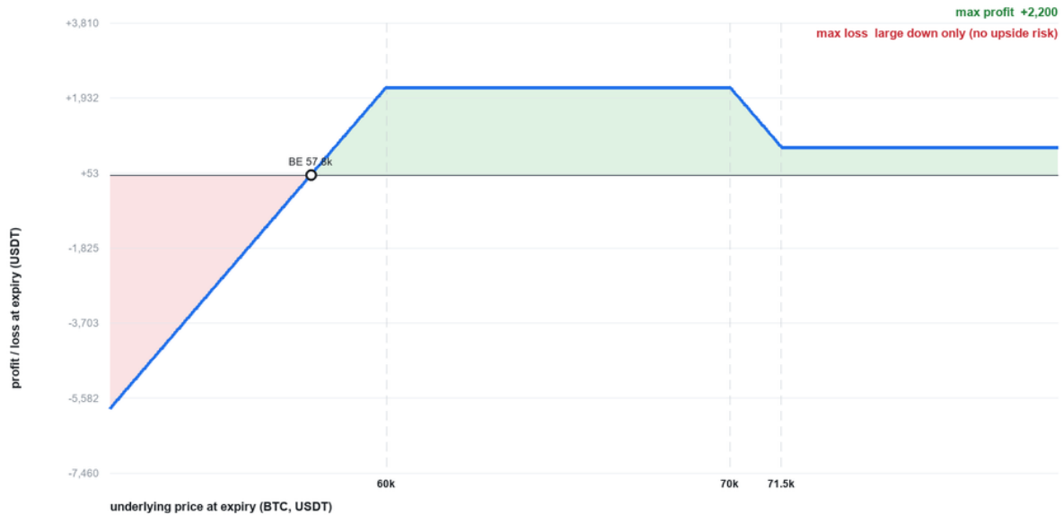
Jade lizard payoff
