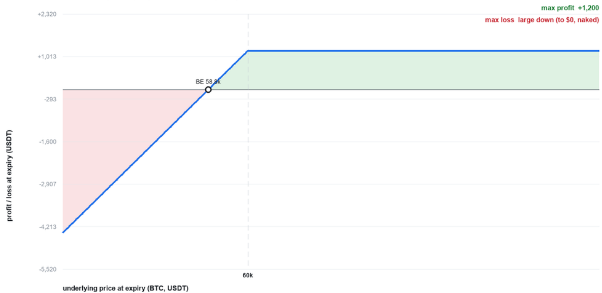
Cash-secured put payoff
