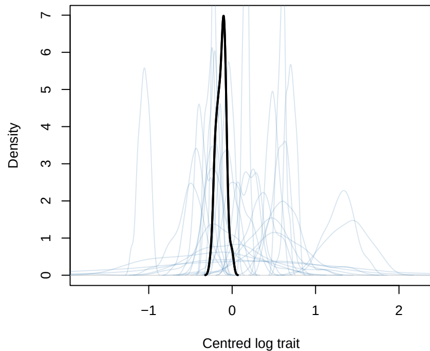
instar_prior1_prior_only mid tenth
