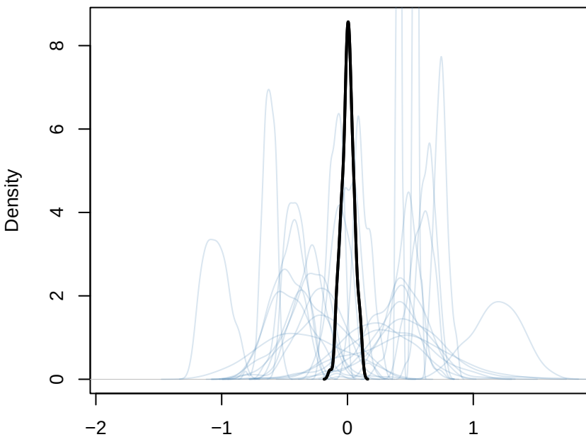
instar_prior1_prior_only fore female
