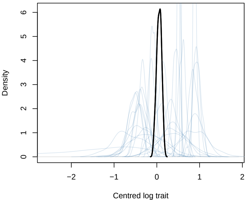
instar_prior1_prior_only hind ninth
