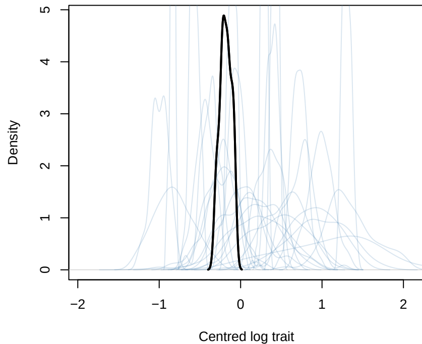
instar_prior1_prior_only eye tenth
