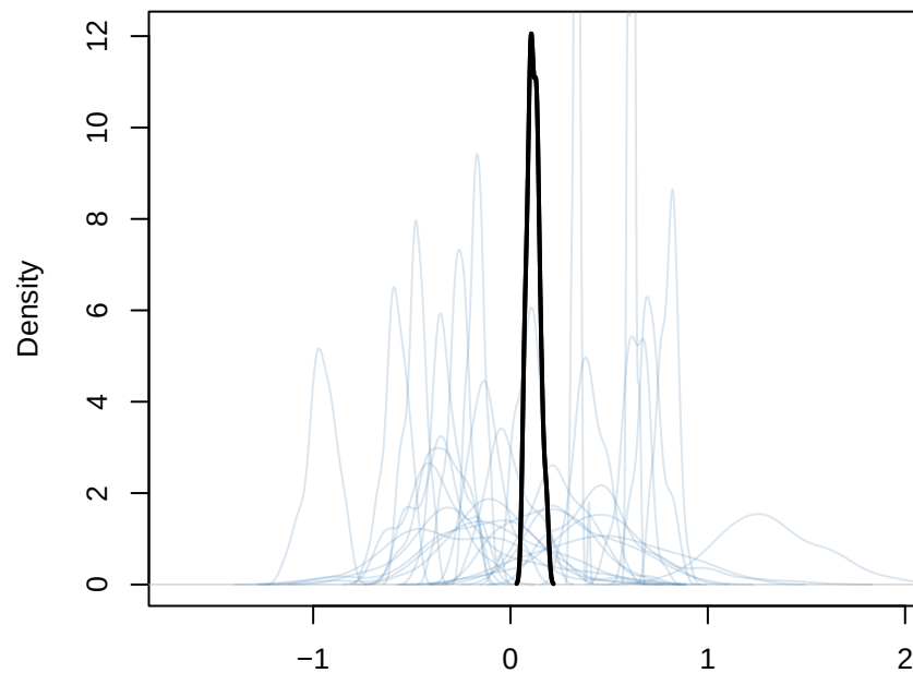
instar_prior1_prior_only fore tenth
