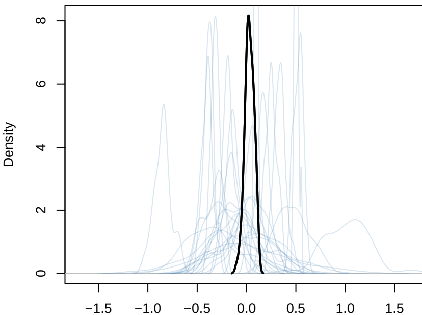
instar_prior1_prior_only fore ninth
