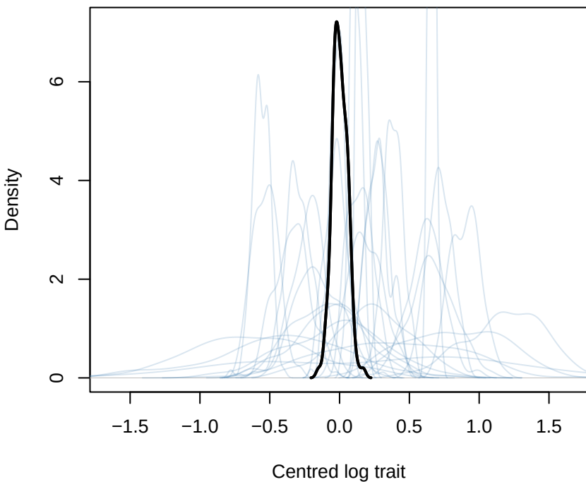
instar_prior1_prior_only earlin ninth
