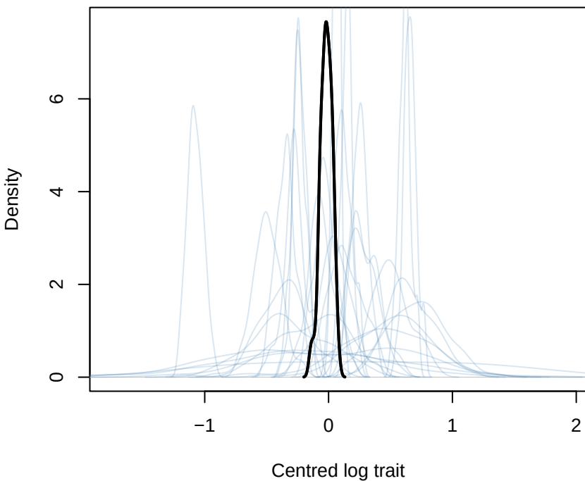
instar_prior1_prior_only mid ninth
