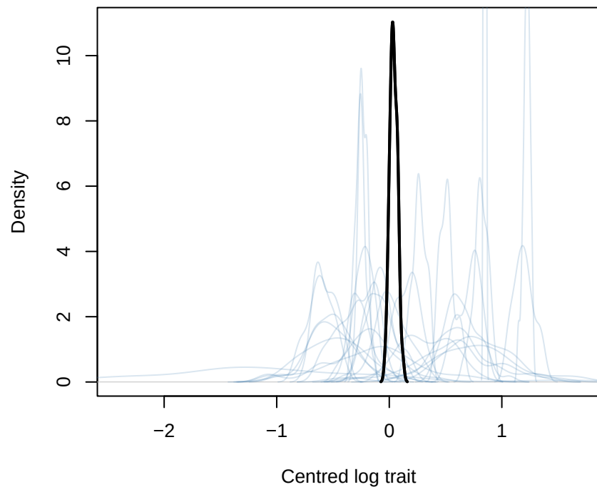
instar_prior1_prior_only hind tenth
