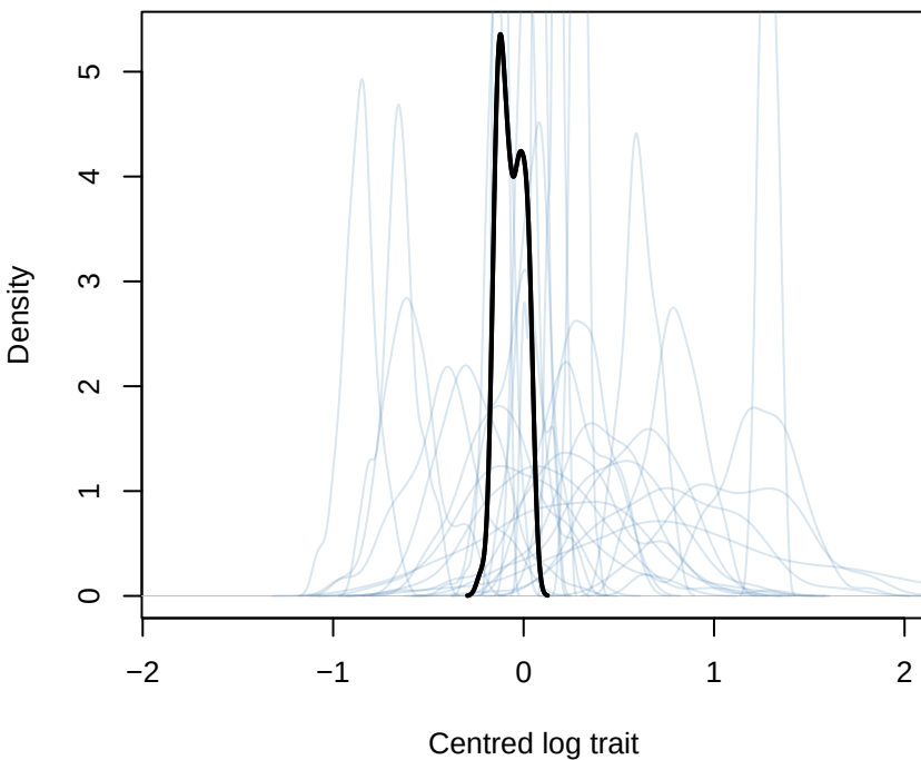
instar_prior1_prior_only eye ninth
