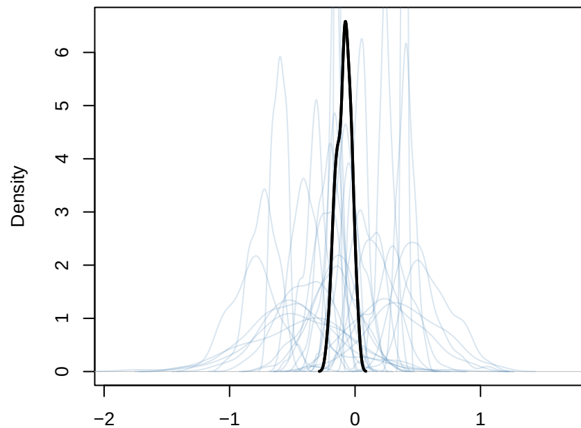
instar_prior1_prior_only fore eighth
