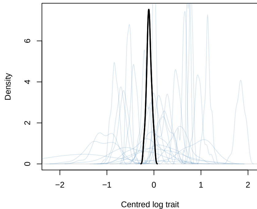
instar_prior1_prior_only earlin tenth
