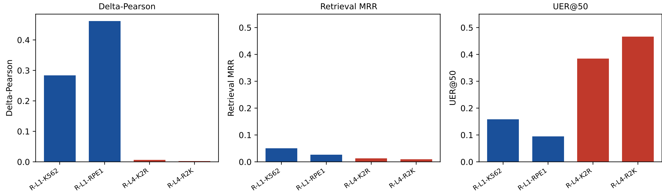
Replogle GEARS R-L1 vs R-L4. R-L4 uses source-context training and target-control-basal prediction.
