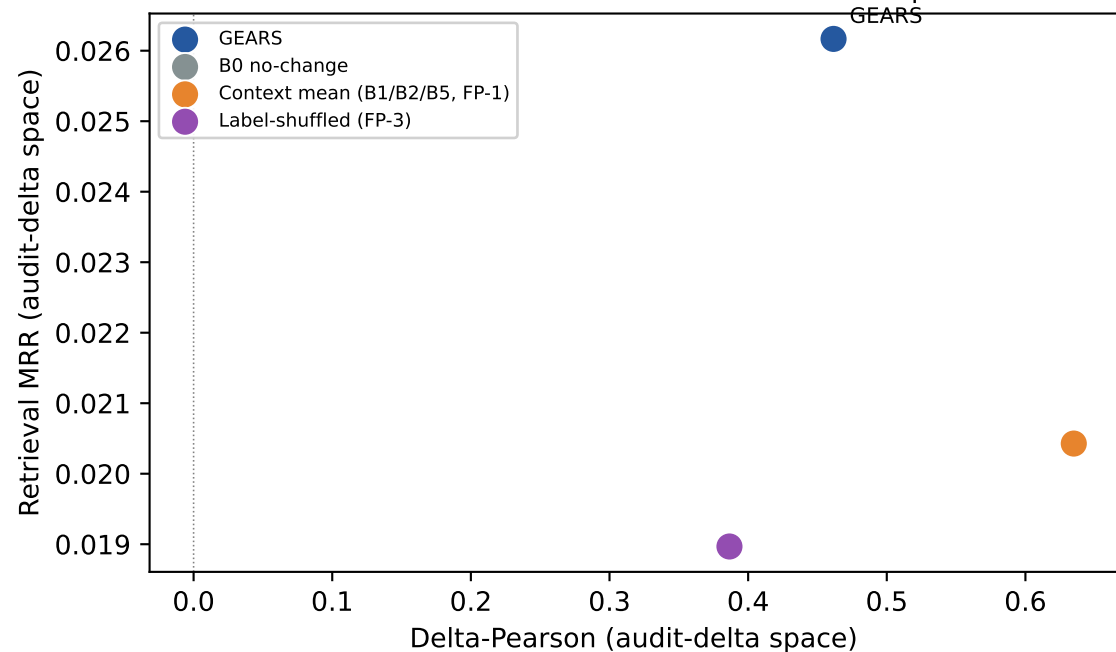
RPE1 R-L1: GEARS vs baselines and falsification probes
