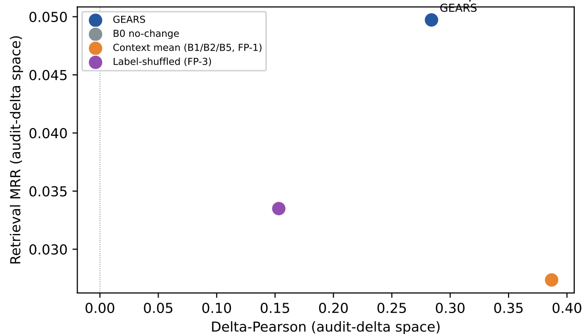
K562 R-L1: GEARS vs baselines and falsification probes
