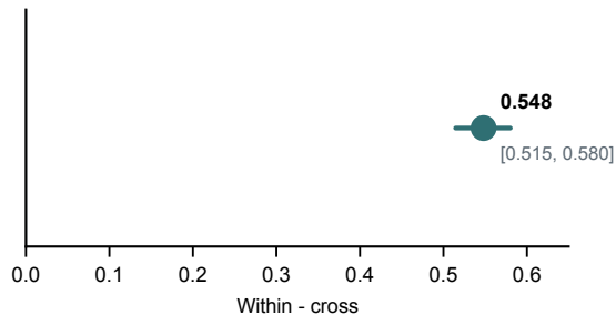
Paired decrease
