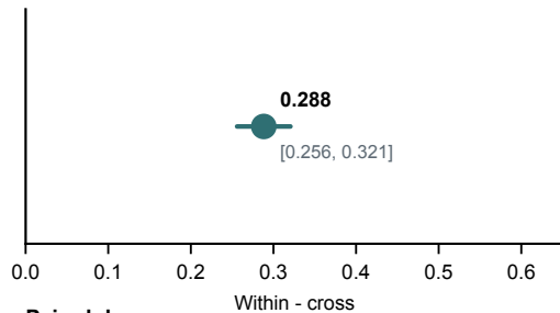
Paired decrease
